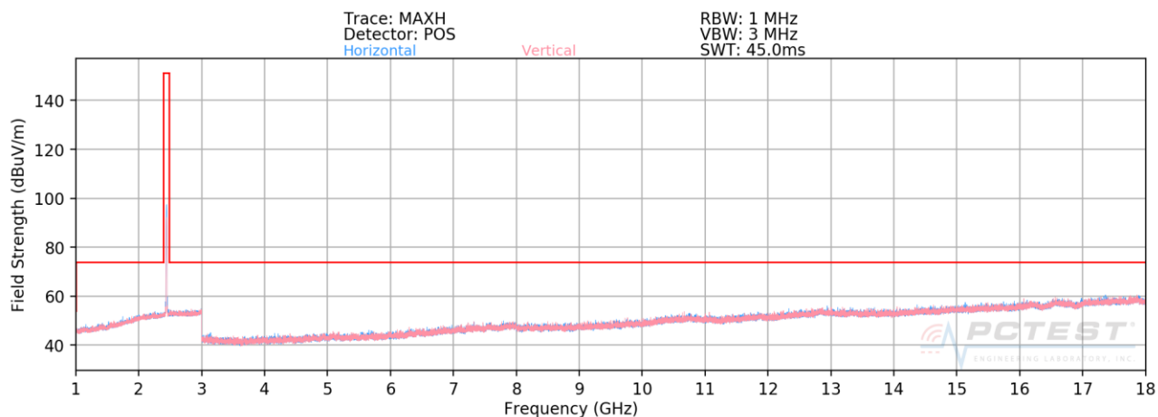
Plot 7-32. Radiated Spurious Plot above 1GHz (802.11b – Ch. 7, Ant. Pol. H & V)
