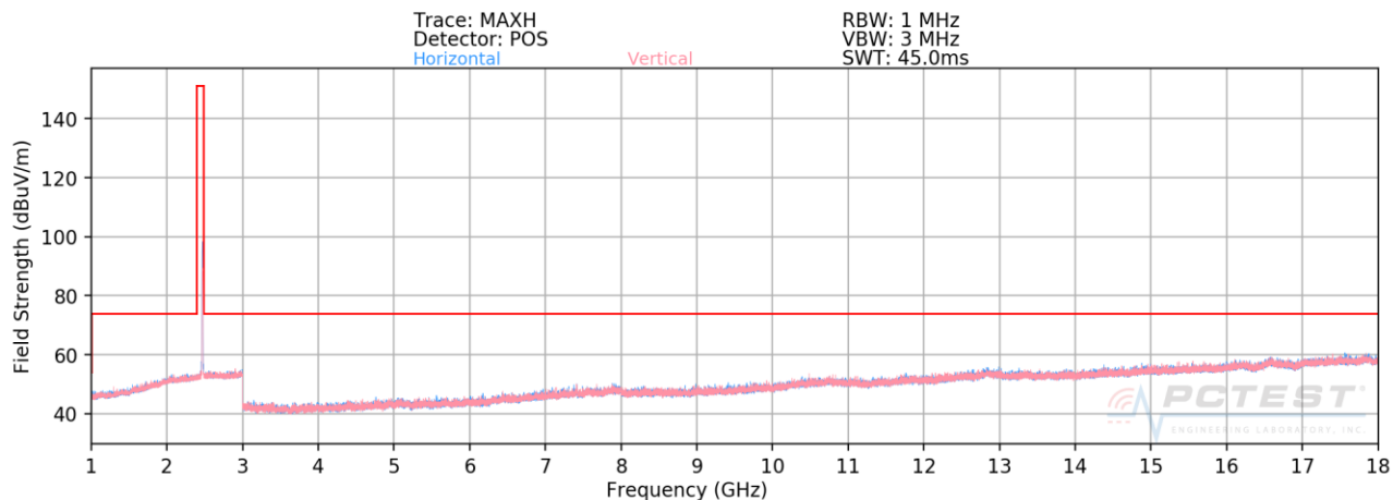
Plot 7-33. Radiated Spurious Plot above 1GHz (802.11b – Ch. 13, Ant. Pol. H & V)
