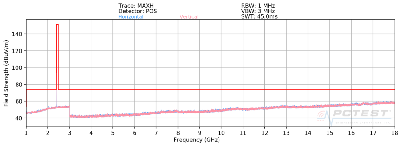
Plot 7-31. Radiated Spurious Plot above 1GHz (802.11b – Ch. 1, Ant. Pol. H & V)
