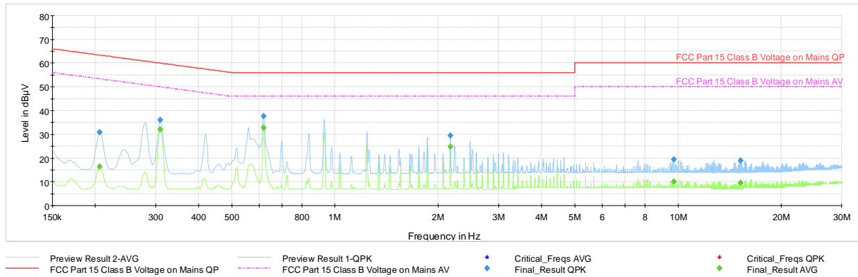
Plot 7-52. Line Conducted Plot with Bluetooth LE (N)
