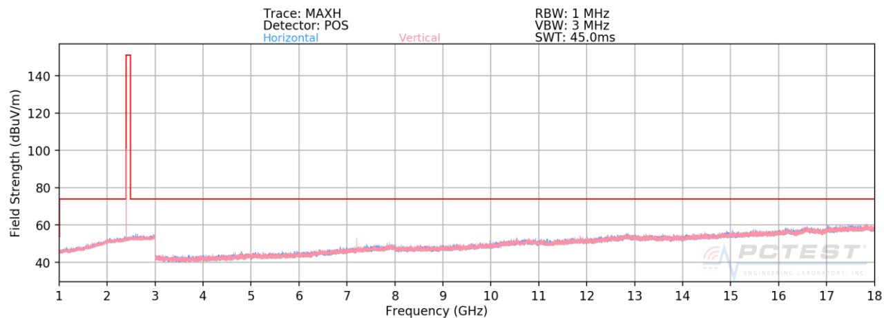
Plot 7-41. Radiated Spurious Plot (1Mbps, ePA – Ch. 0, Ant. Pol. H & V)
