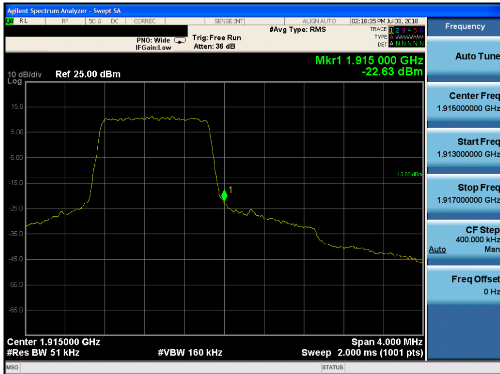
Plot 7-220. Upper Band Edge Plot (Band 25 - 1.4MHz QPSK - Full RB Configuration)
