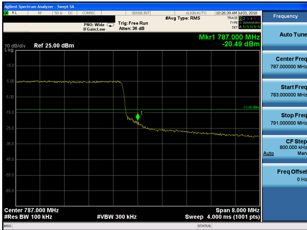
Plot 7-176. Upper Band Edge Plot (Band 13 - 10.0MHz QPSK - Full RB Configuration)
