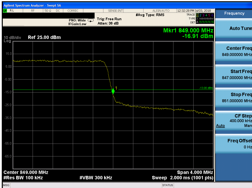
Plot 7-181. Upper Band Edge Plot (Band 26 - 3.0MHz QPSK - Full RB Configuration)
