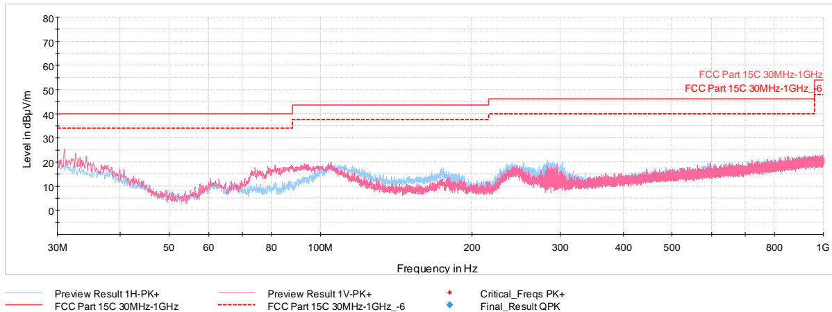
Plot 7-9. Radiated Spurious Plot 30MHz – 1GHz (Reader 100 Ask 1 out of 4, Pol. H & V)
