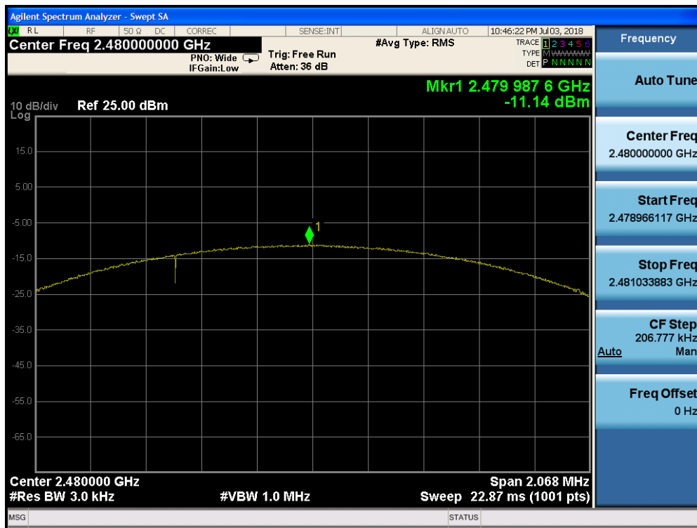
Plot 7-24. Power Spectral Density Plot (Bluetooth (LE), 2Mbps, iPA – Ch. 39)
