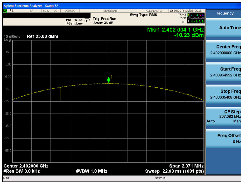
Plot 7-22. Power Spectral Density Plot (Bluetooth (LE), 2Mbps, iPA – Ch. 0)
