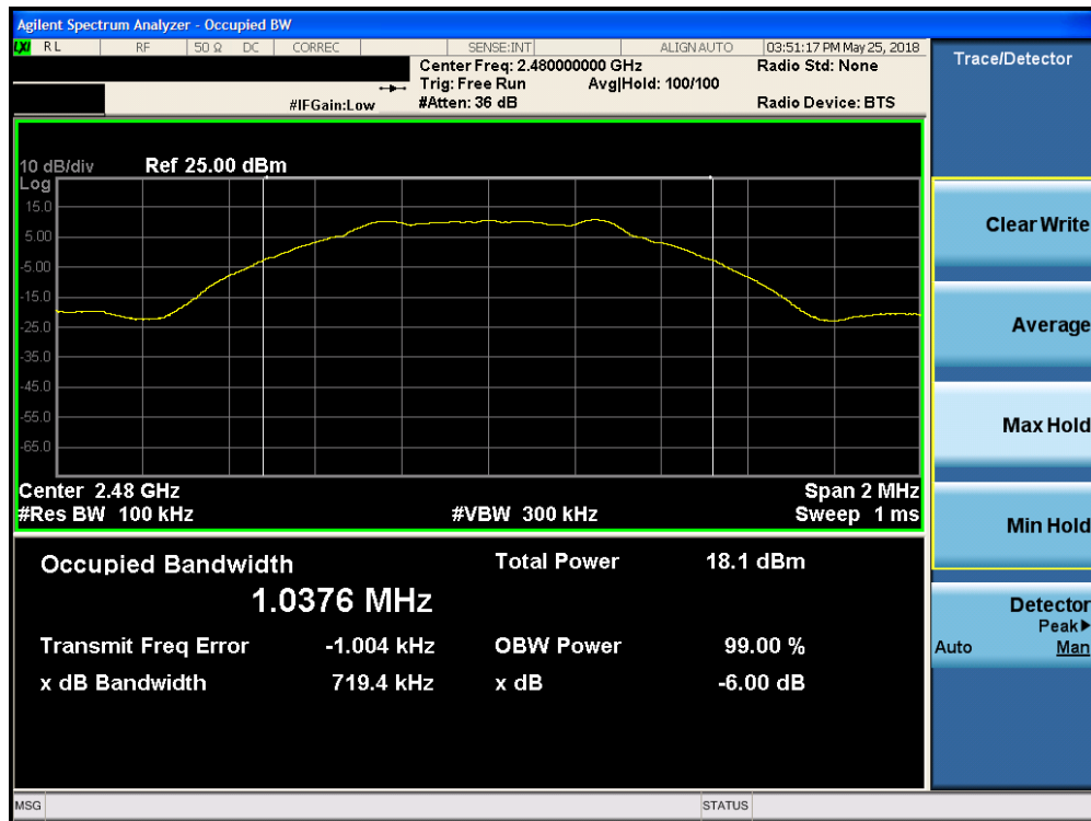
Plot 7-9. 6dB Bandwidth Plot (Bluetooth (LE), 1Mbps, iPA – Ch. 39)
