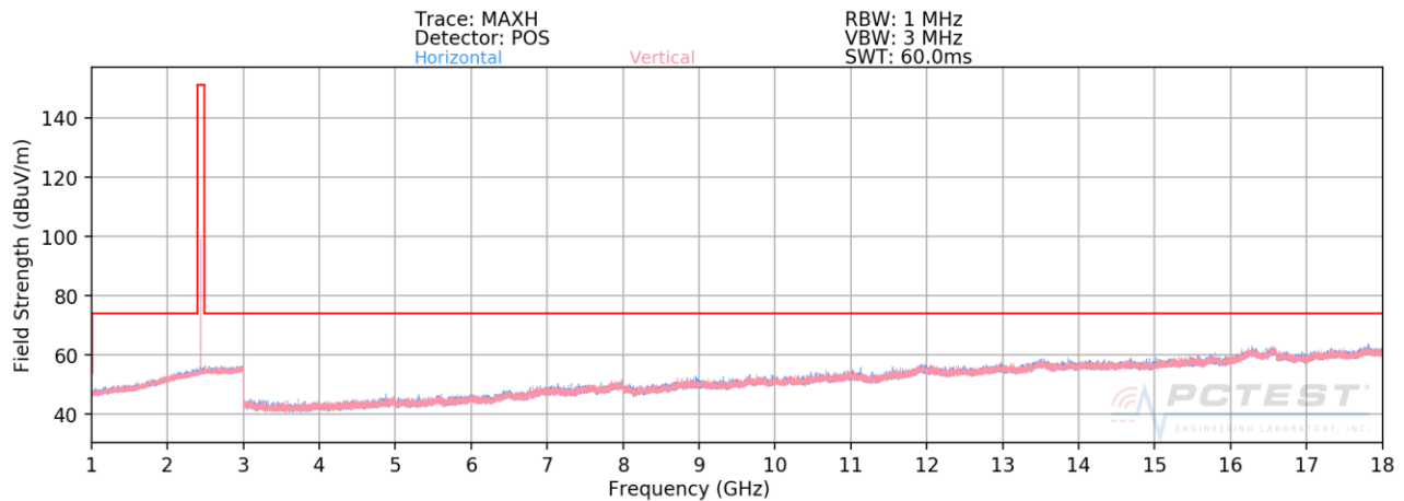
Plot 7-42. Radiated Spurious Plot Above 1GHz (1Mbps, ePA – Ch. 19, Ant. Pol. H & V)
