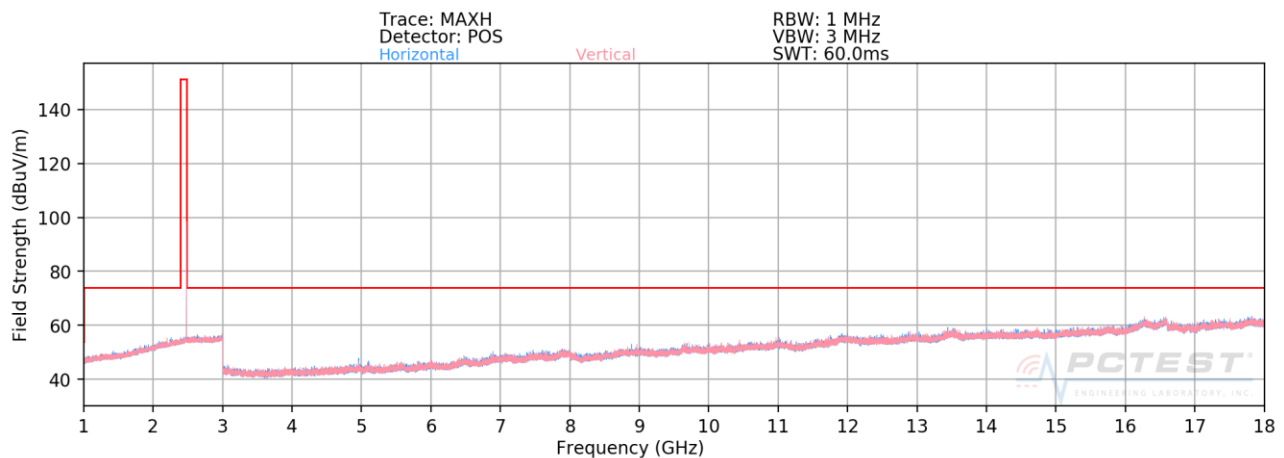
Plot 7-43. Radiated Spurious Plot Above 1GHz (1Mbps, ePA – Ch. 39, Ant. Pol. H & V)
