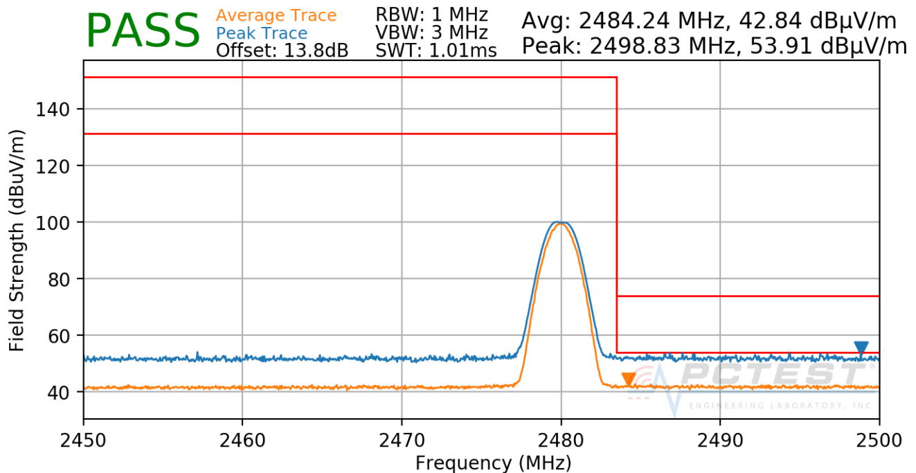
Plot 7-48. Radiated Restricted Upper Band Edge Measurement (Average & Peak)
