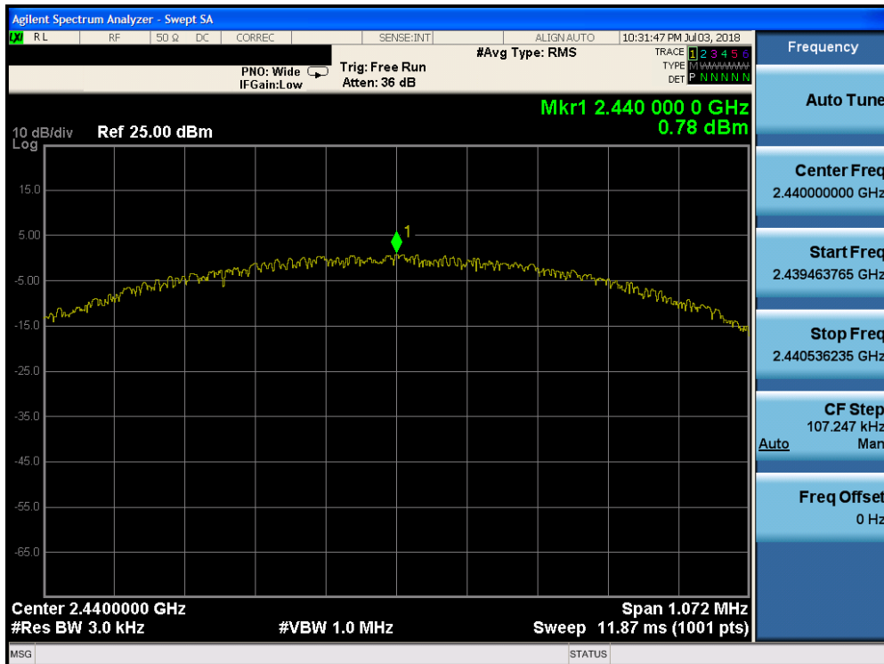
Plot 7-14. Power Spectral Density Plot (Bluetooth (LE), 1Mbps, ePA – Ch. 19)
