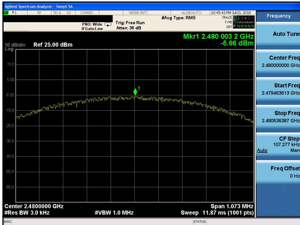
Plot 7-18. Power Spectral Density Plot (Bluetooth (LE), 1Mbps, iPA – Ch. 39)
