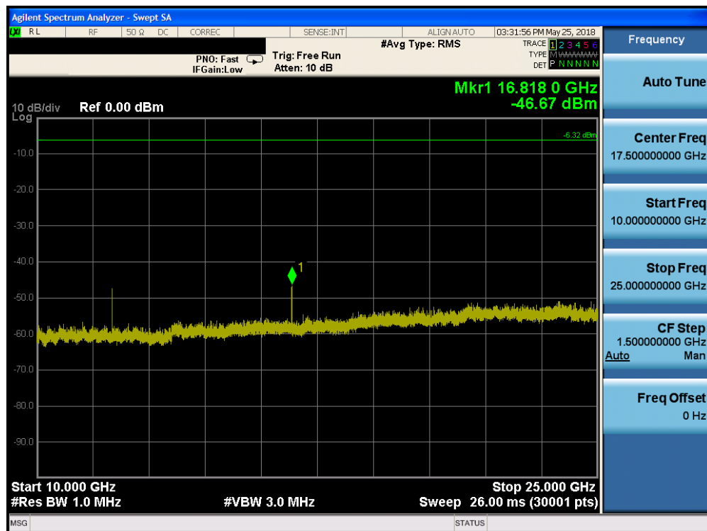
Plot 7-36. Conducted Spurious Plot (Bluetooth (LE), 2Mbps, ePA – Ch. 0)
