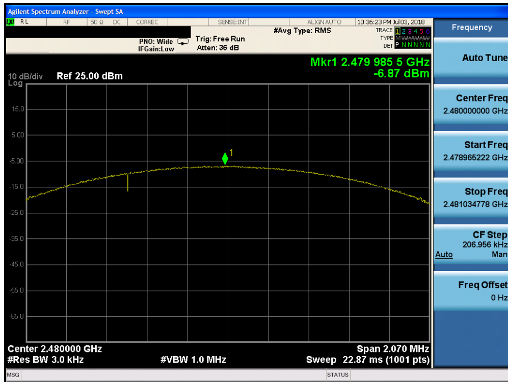
Plot 7-21. Power Spectral Density Plot (Bluetooth (LE), 2Mbps, ePA – Ch. 39)
