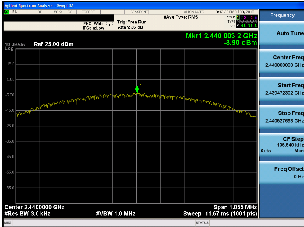
Plot 7-17. Power Spectral Density Plot (Bluetooth (LE), 1Mbps, iPA – Ch. 19)
