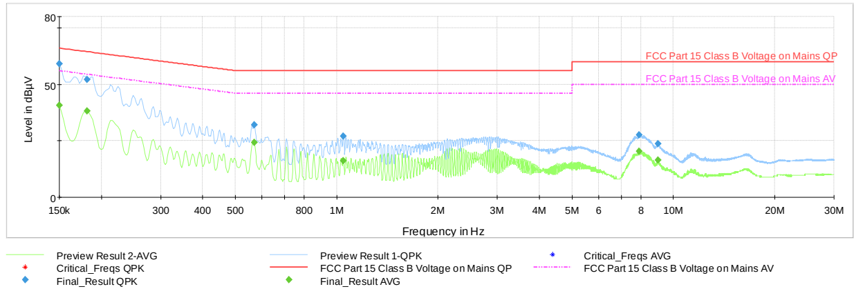
Plot 7-52. Line Conducted Plot with Bluetooth LE (N, with WCP + Laptop))
