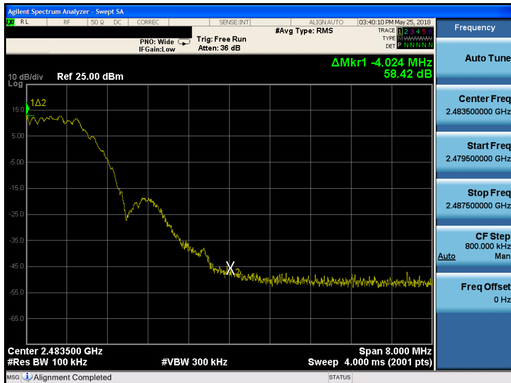
Plot 7-28. Band Edge Plot (Bluetooth (LE), 2Mbps, ePA – Ch. 39)
