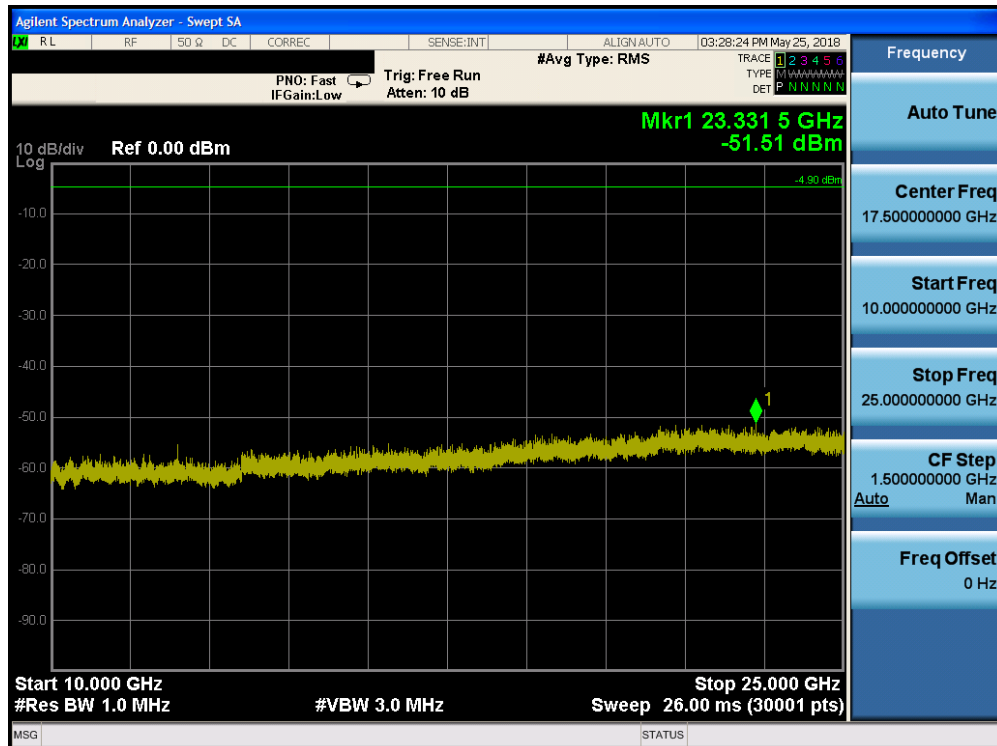
Plot 7-34. Conducted Spurious Plot (Bluetooth (LE), 1Mbps, ePA – Ch. 39)
