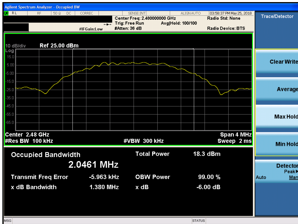
Plot 7-12. 6dB Bandwidth Plot (Bluetooth (LE), 2Mbps, iPA – Ch. 39)
