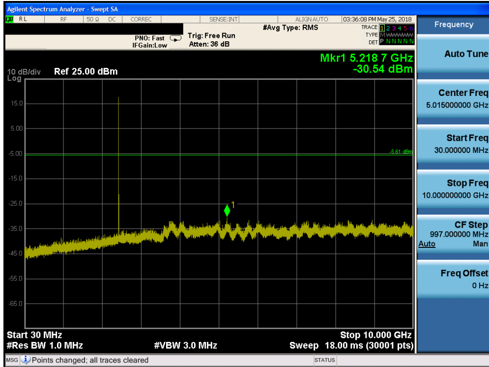
Plot 7-37. Conducted Spurious Plot (Bluetooth (LE), 2Mbps, ePA – Ch. 19)
