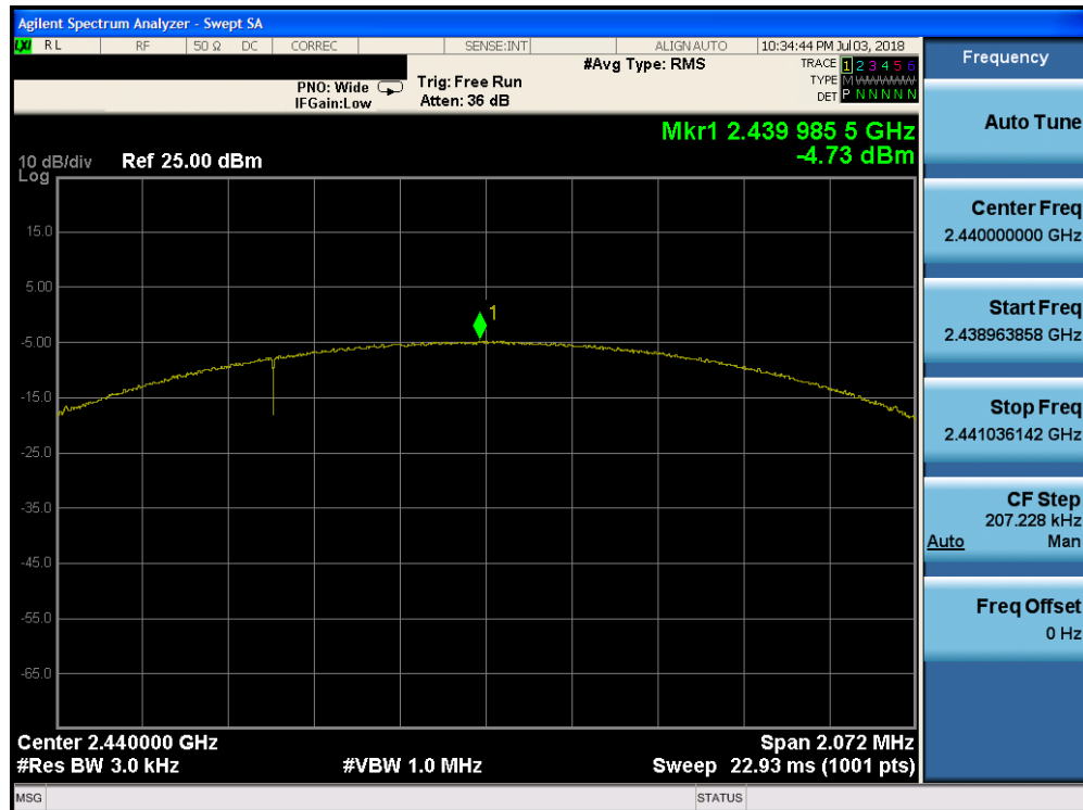
Plot 7-20. Power Spectral Density Plot (Bluetooth (LE), 2Mbps, ePA – Ch. 19)
