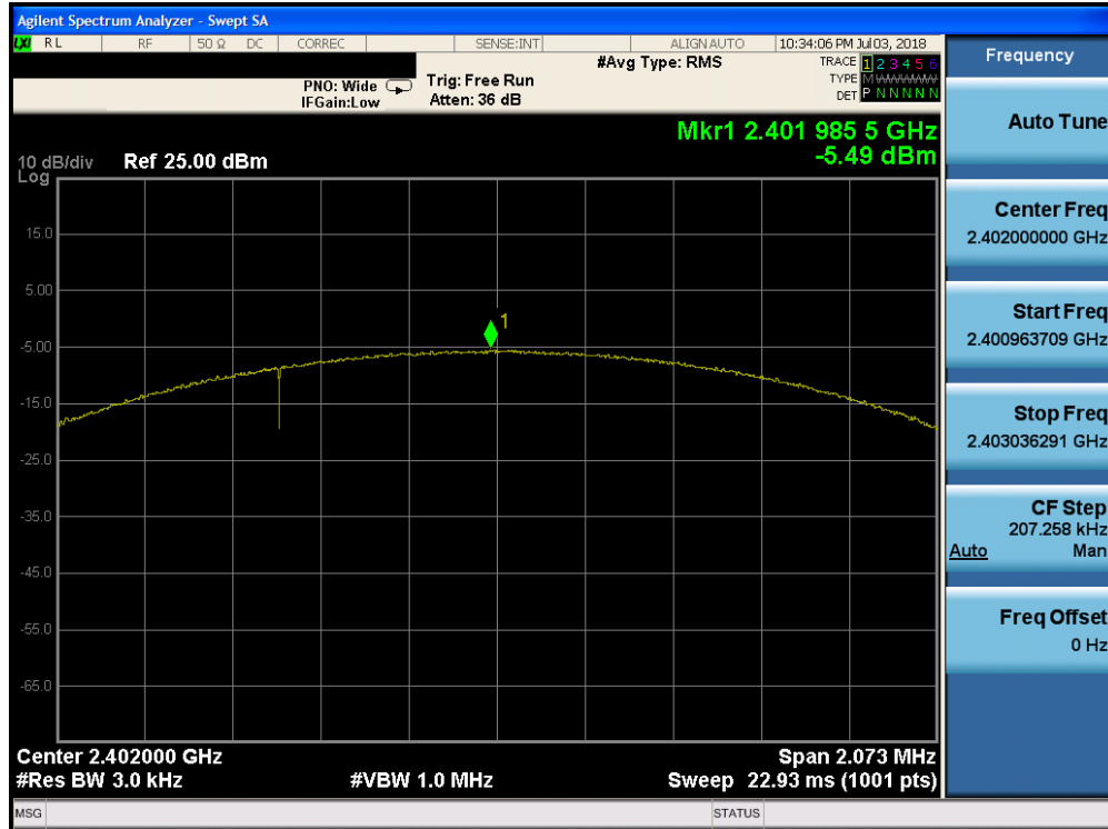
Plot 7-19. Power Spectral Density Plot (Bluetooth (LE), 2Mbps, ePA – Ch. 0)
