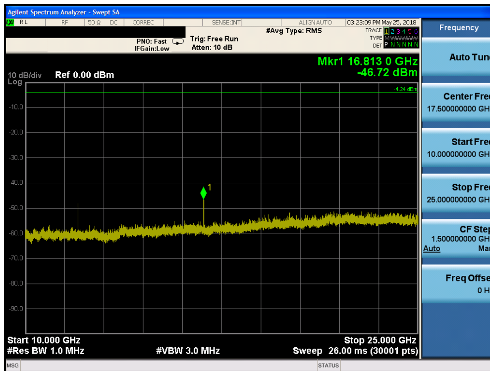
Plot 7-30. Conducted Spurious Plot (Bluetooth (LE), 1Mbps, ePA – Ch. 0)
