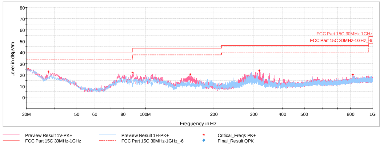
Plot 7-50. Radiated Spurious Plot below 1GHz (1Mbps ePA, Pol. H & V, with WCP + Adapter)
