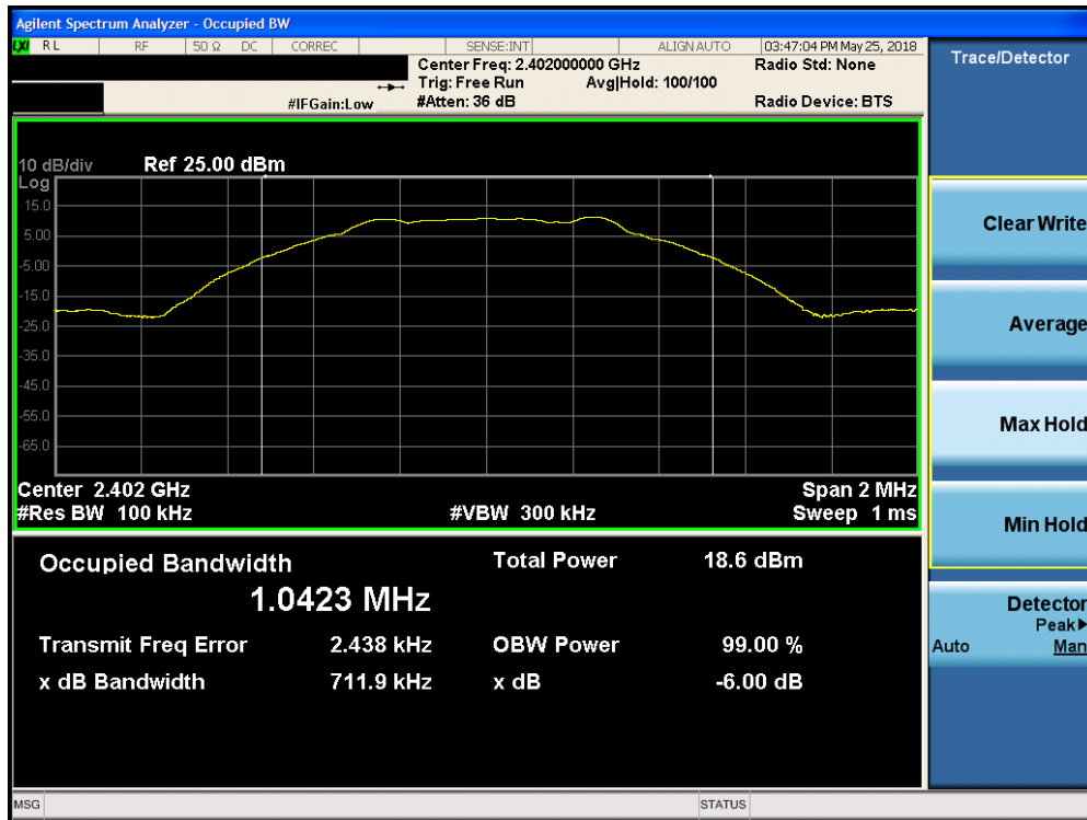
Plot 7-7. 6dB Bandwidth Plot (Bluetooth (LE), 1Mbps, iPA – Ch. 0)
