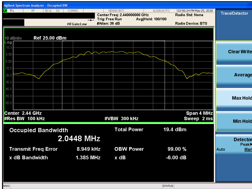
Plot 7-11. 6dB Bandwidth Plot (Bluetooth (LE), 2Mbps, iPA – Ch. 19)
