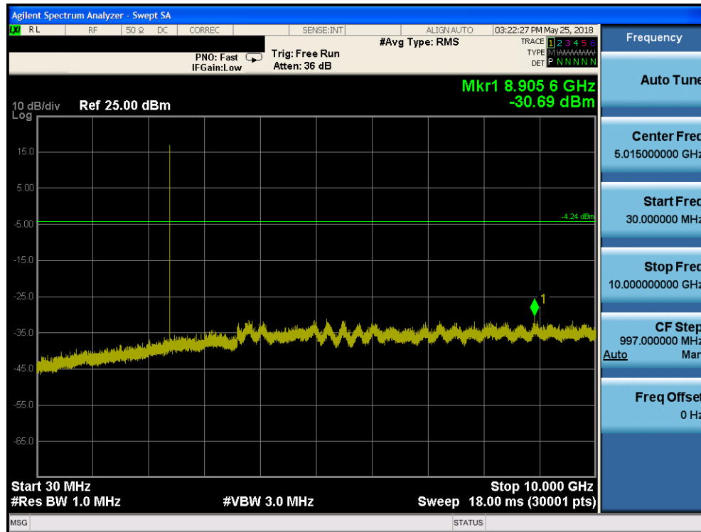
Plot 7-29. Conducted Spurious Plot (Bluetooth (LE), 1Mbps, ePA – Ch. 0)
