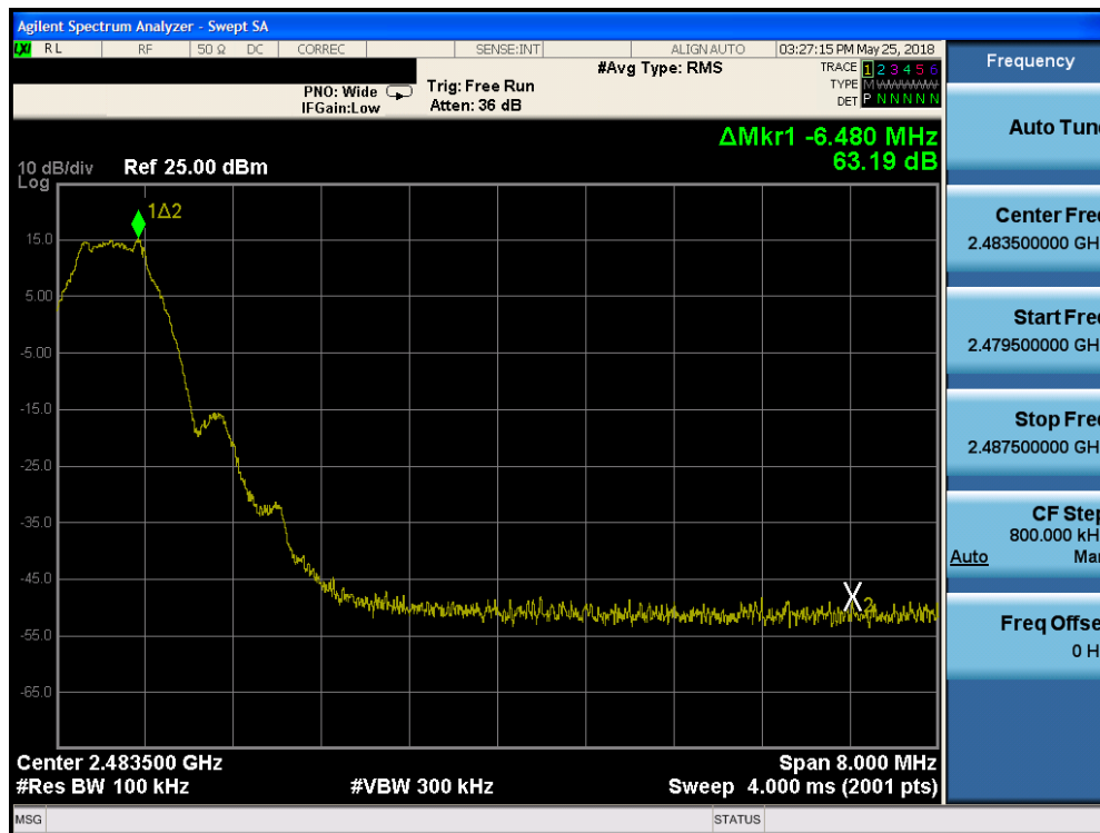
Plot 7-26. Band Edge Plot (Bluetooth (LE), 1Mbps, ePA – Ch. 39)
