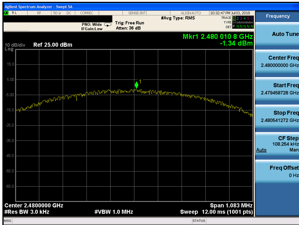
Plot 7-15. Power Spectral Density Plot (Bluetooth (LE), 1Mbps, ePA – Ch. 39)
