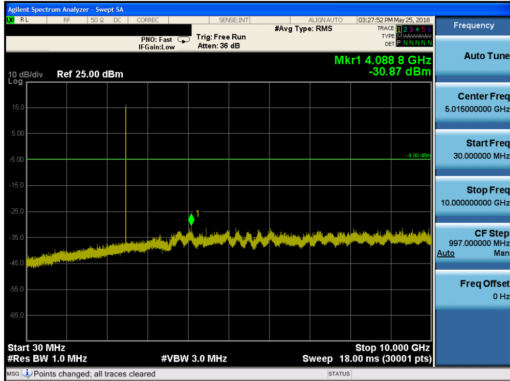
Plot 7-33. Conducted Spurious Plot (Bluetooth (LE), 1Mbps, ePA – Ch. 39)
