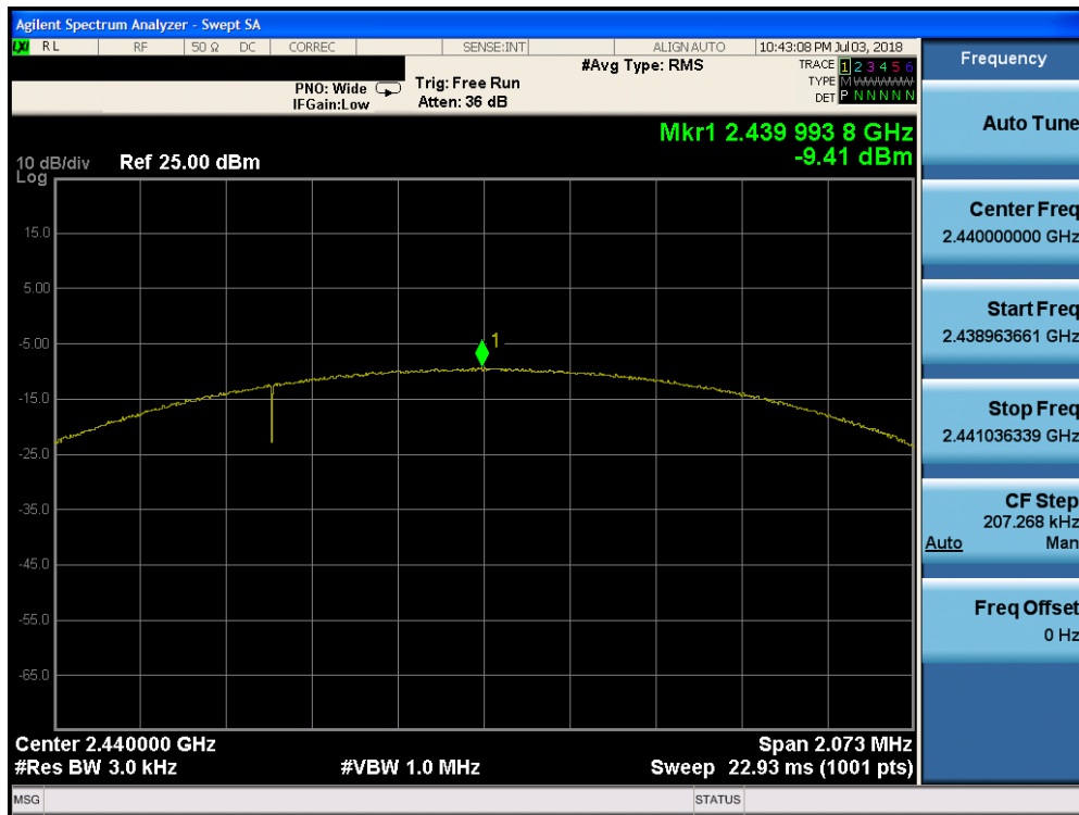
Plot 7-23. Power Spectral Density Plot (Bluetooth (LE), 2Mbps, iPA – Ch. 19)
