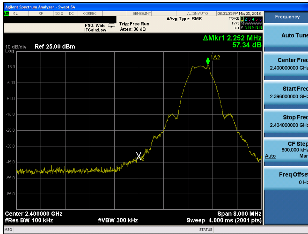
Plot 7-25. Band Edge Plot (Bluetooth (LE), 1Mbps, ePA – Ch. 0)
