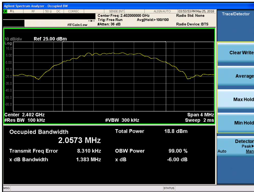
Plot 7-10. 6dB Bandwidth Plot (Bluetooth (LE), 2Mbps, iPA – Ch. 0)
