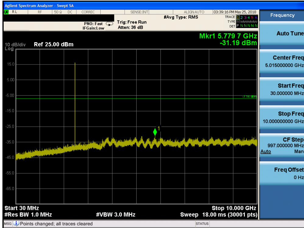
Plot 7-39. Conducted Spurious Plot (Bluetooth (LE), 2Mbps, ePA – Ch. 39)
