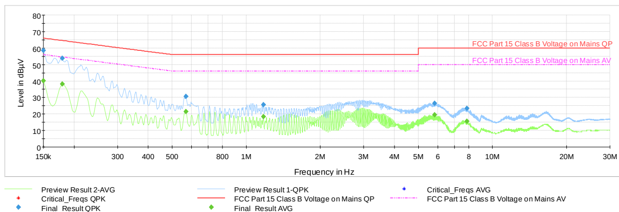
Plot 7-51. Line Conducted Plot with Bluetooth LE (L1, with WCP + Laptop)
