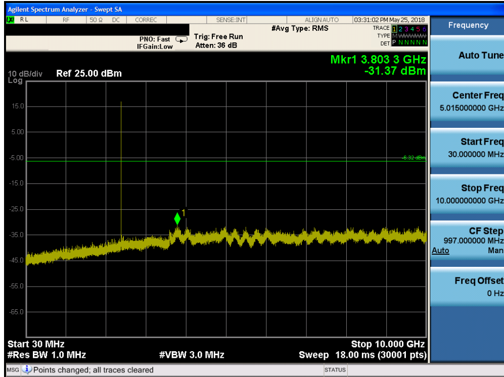
Plot 7-35. Conducted Spurious Plot (Bluetooth (LE), 2Mbps, ePA – Ch. 0)
