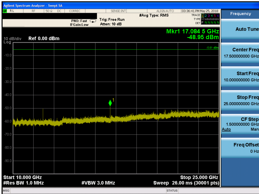
Plot 7-38. Conducted Spurious Plot (Bluetooth (LE), 2Mbps, ePA – Ch. 19)
