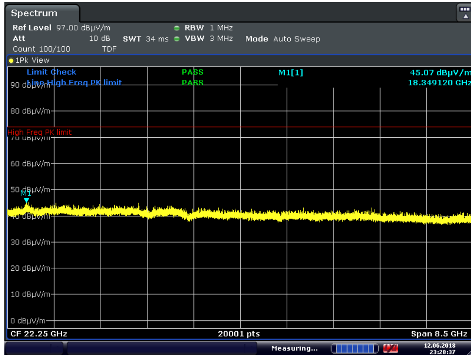
Plot 7-44. Radiated Spurious Plot Above 18GHz (1Mbps, ePA, Ant. Pol. H)
