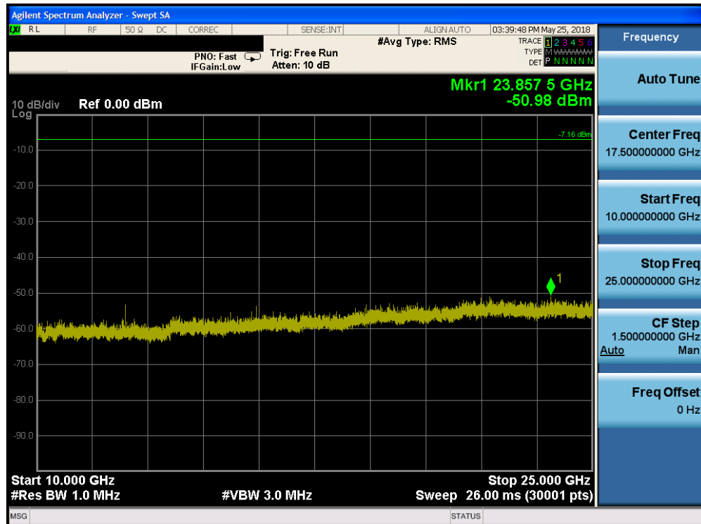
Plot 7-40. Conducted Spurious Plot (Bluetooth (LE), 2Mbps, ePA – Ch. 39)
