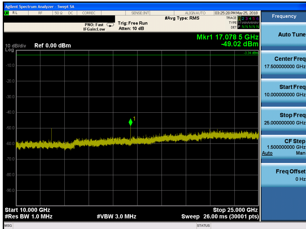
Plot 7-32. Conducted Spurious Plot (Bluetooth (LE), 1Mbps, ePA – Ch. 19)
