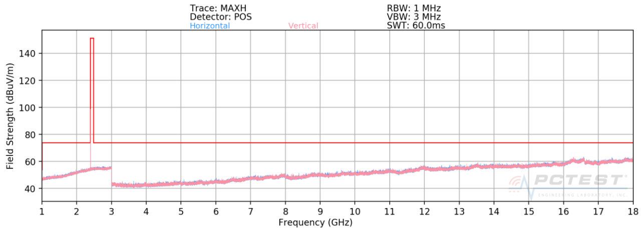
Plot 7-41. Radiated Spurious Plot Above 1GHz (1Mbps, ePA – Ch. 0, Ant. Pol. H & V)
