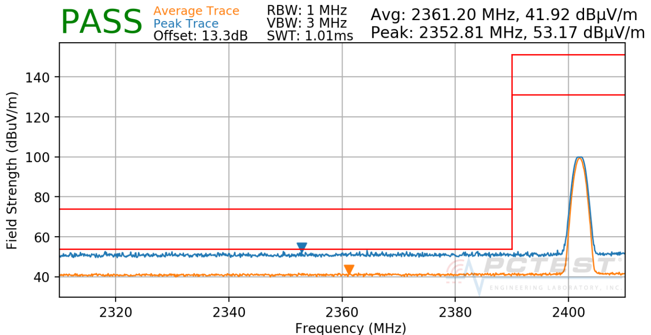
Plot 7-46. Radiated Restricted Lower Band Edge Measurement (Average & Peak)
