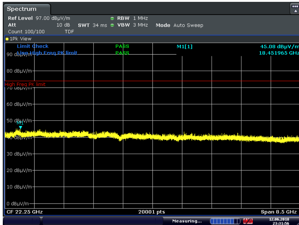
Plot 7-45. Radiated Spurious Plot Above 18GHz (1Mbps, ePA, Ant. Pol. V)
