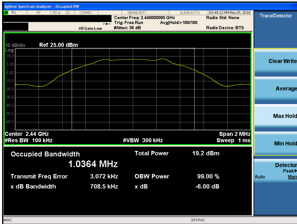
Plot 7-8. 6dB Bandwidth Plot (Bluetooth (LE), 1Mbps, iPA – Ch. 19)
