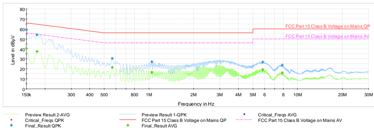
Plot 7-59. Line Conducted Plot with Bluetooth HDR (L1, with WCP + Laptop)
