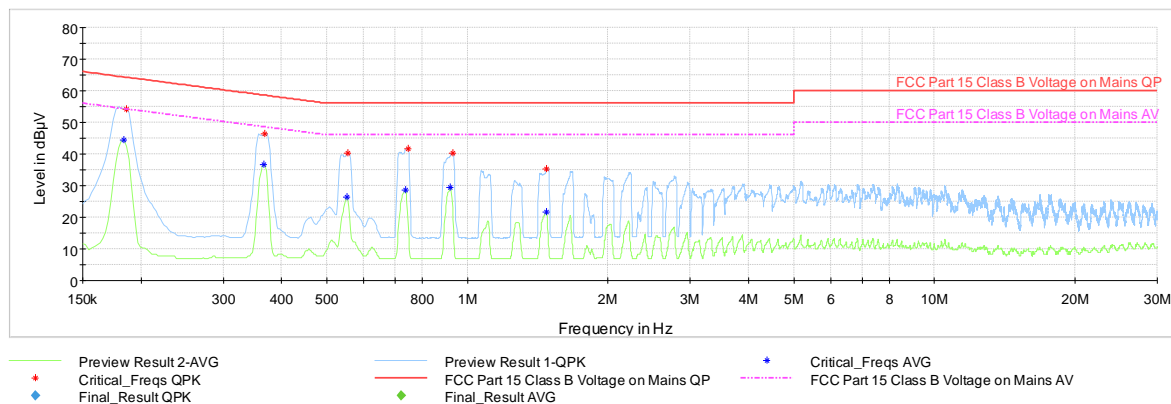
Plot 7-30. Line Conducted Plot with Bluetooth LE with AC Adapter (N)
