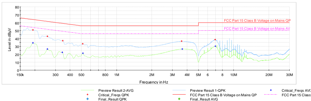
Plot 7-32. Line Conducted Plot with Bluetooth LE with Laptop (N)
