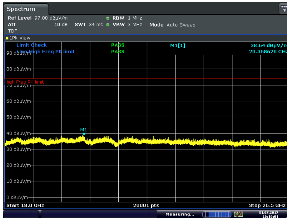
Plot 7-21. Radiated Spurious Plot above 18GHz (Pol. H)
