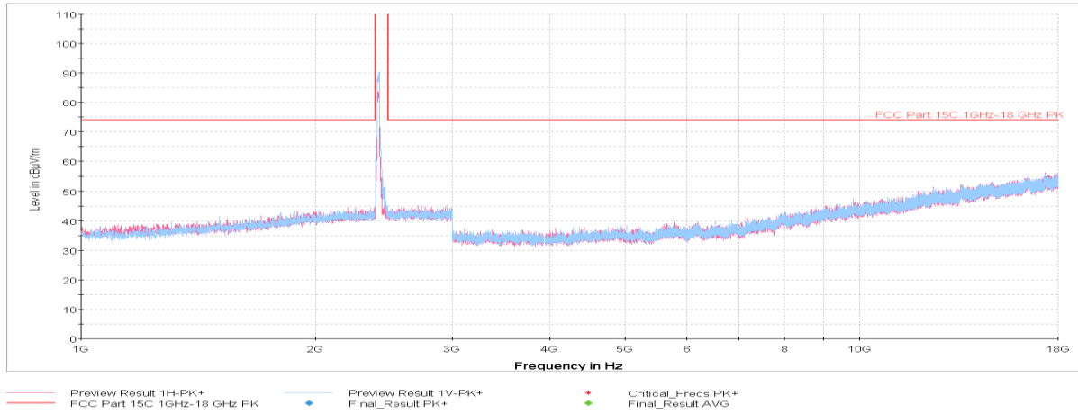
Plot 7-37. Radiated Spurious Plot above 1GHz (802.11b – Ch. 1, Ant. Pol. H & V)
