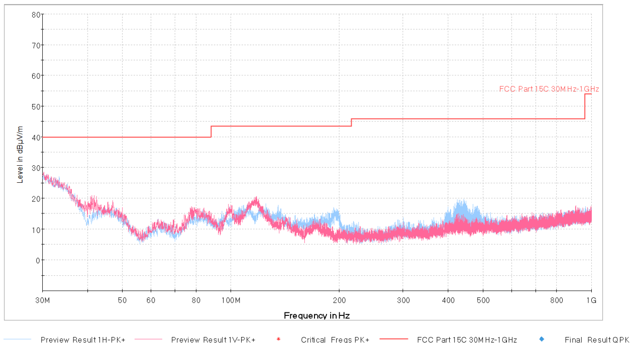
Plot 7-50. Radiated Spurious Plot below 1GHz (802.11b – Ch. 6, Pol. H & V)
