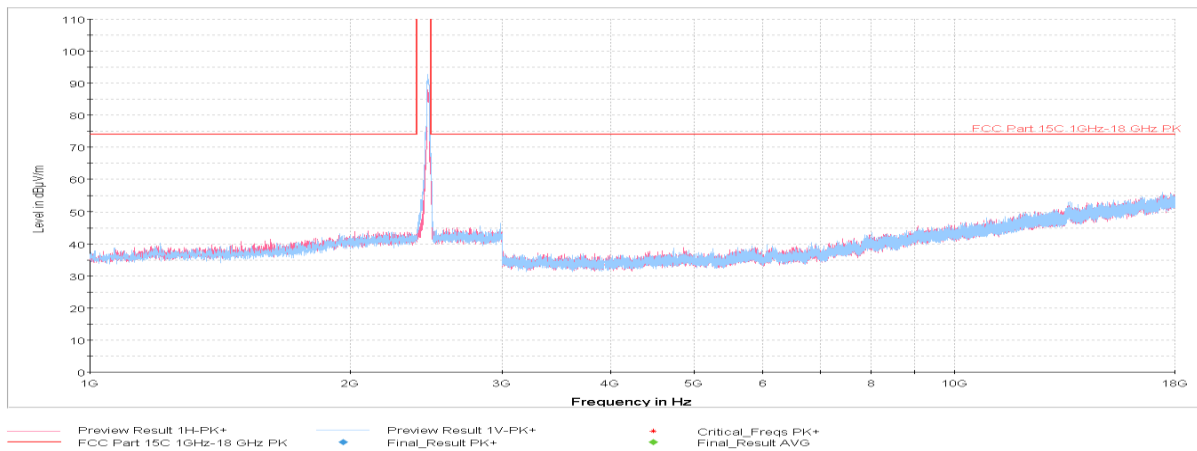
Plot 7-39. Radiated Spurious Plot above 1GHz (802.11b – Ch. 11, Ant. Pol. H & V)
