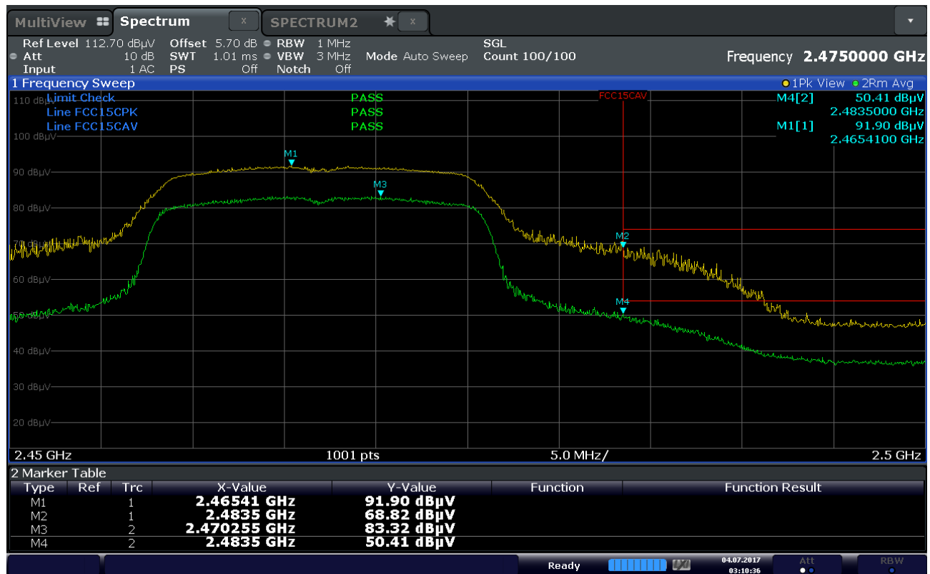
Plot 7-48. Radiated Restricted Upper Band Edge Measurement (Average & Peak)
