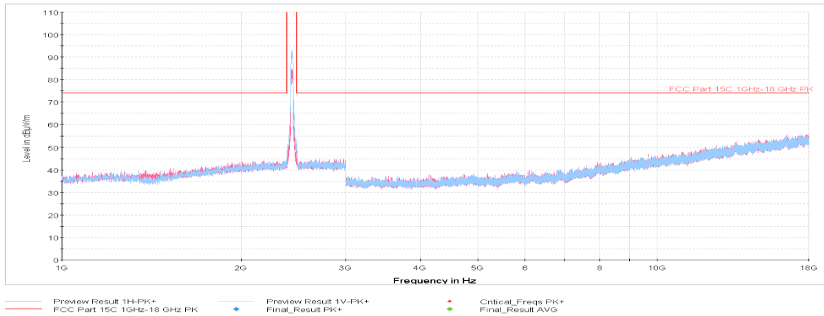
Plot 7-38. Radiated Spurious Plot above 1GHz (802.11b – Ch. 6, Ant. Pol. H & V)
