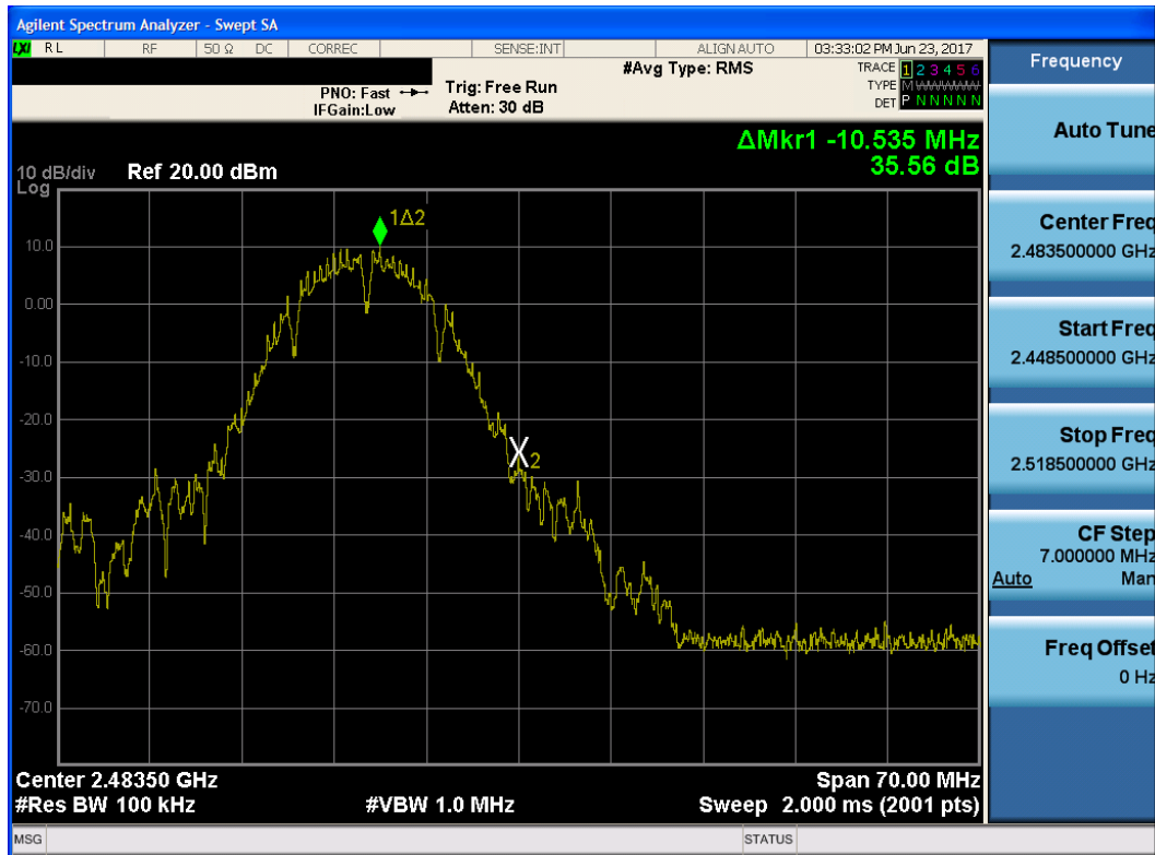
Plot 7-22. Band Edge Plot (802.11b – Ch. 13)
