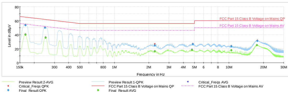
Plot 7-52. Line Conducted Plot with 802.11b (N)
