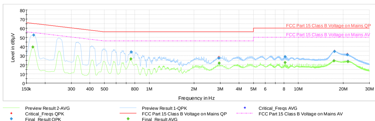
Plot 7-51. Line Conducted Plot with 802.11b (L1)
