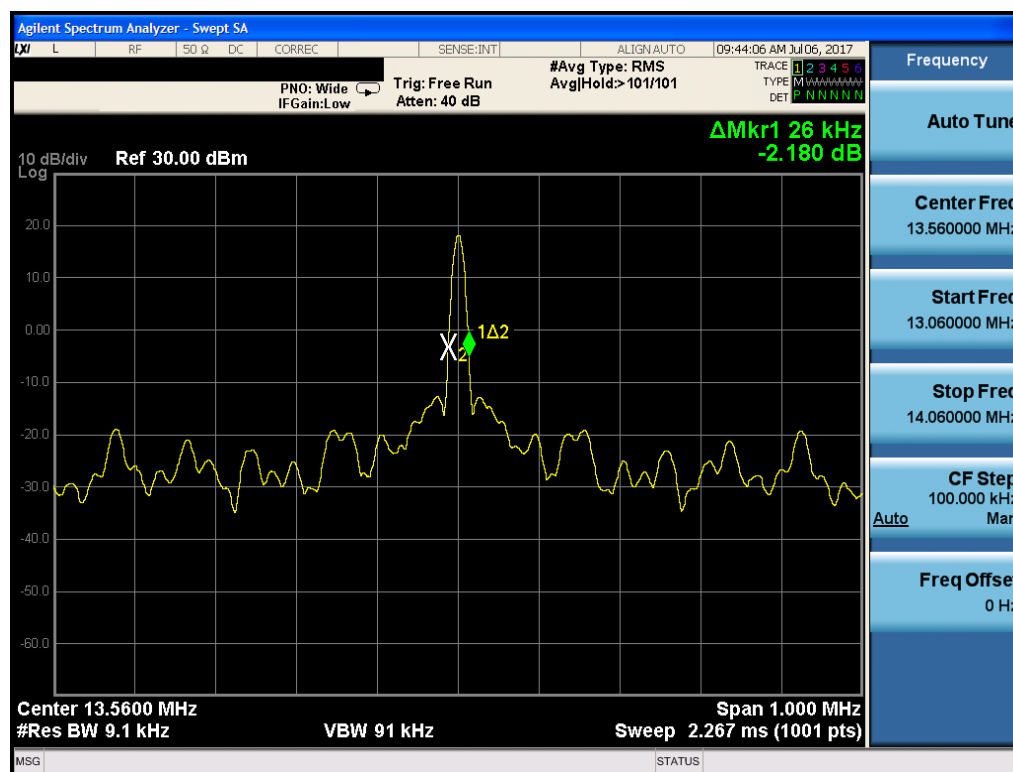
Figure 7-3. 20dB Bandwidth Plot (CE B 848kbps)
