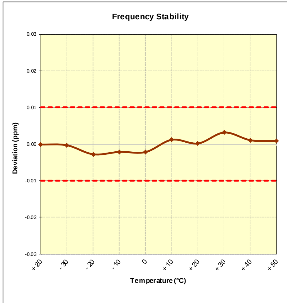
Figure 7-11. Frequency Stability Plot (Reader 100% Ask 1 out of 256)
