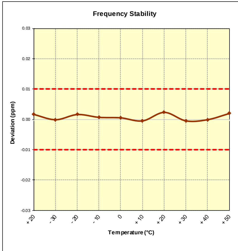
Figure 7-9. Frequency Stability Plot (CE F 424kbps)
