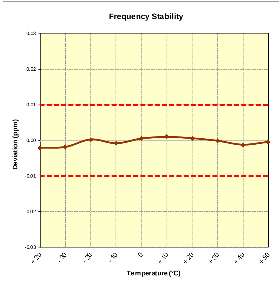
Figure 7-10. Frequency Stability Plot (Reader 100% Ask 1 out of 4)
