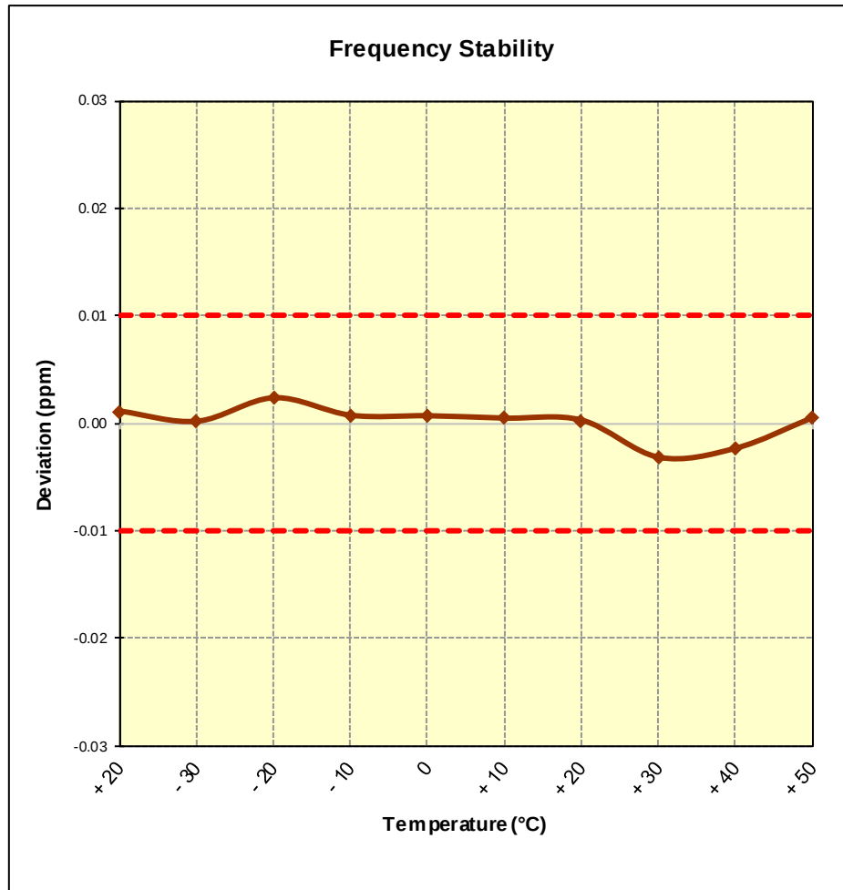
Figure 7-8. Frequency Stability Plot (CE B 848kbps)
