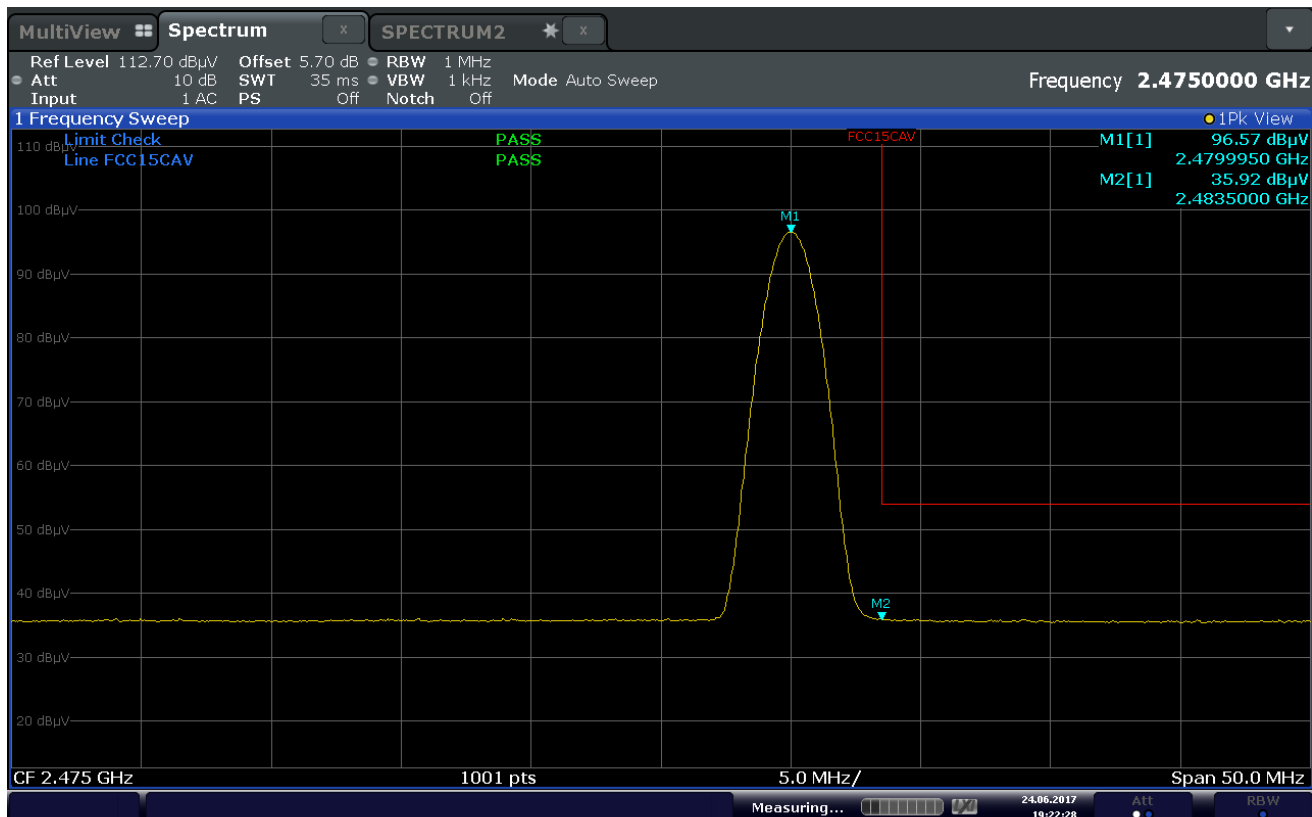
Plot 7-70. Radiated Restricted Upper Band Edge Measurement (Average)
