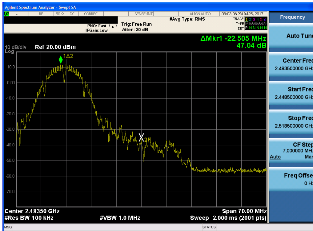
Plot 7-20. Band Edge Plot (802.11b – Ch. 11)
