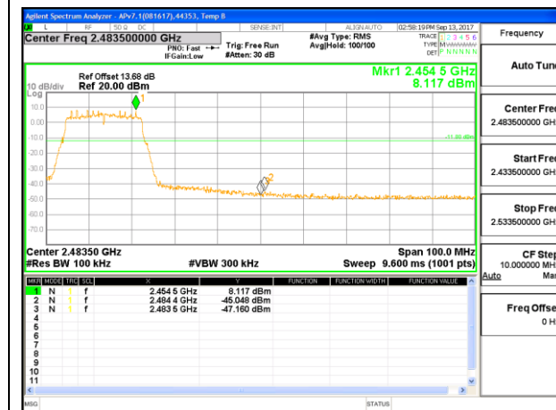
HIGH CHANNEL 8 BANDEDGE ANT A
