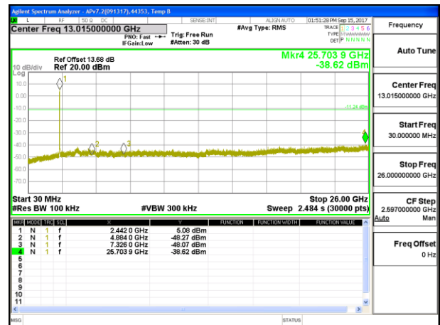
OUT-OF-BAND HIGH CHANNEL 7 ANT A
