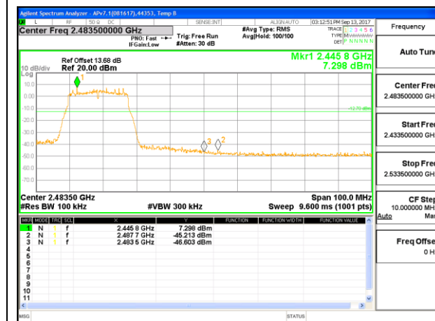
HIGH CHANNEL 9 BANDEDGE ANT A
