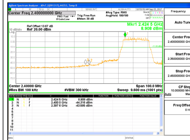
LOW CHANNEL 5 BANDEDGE ANT A
