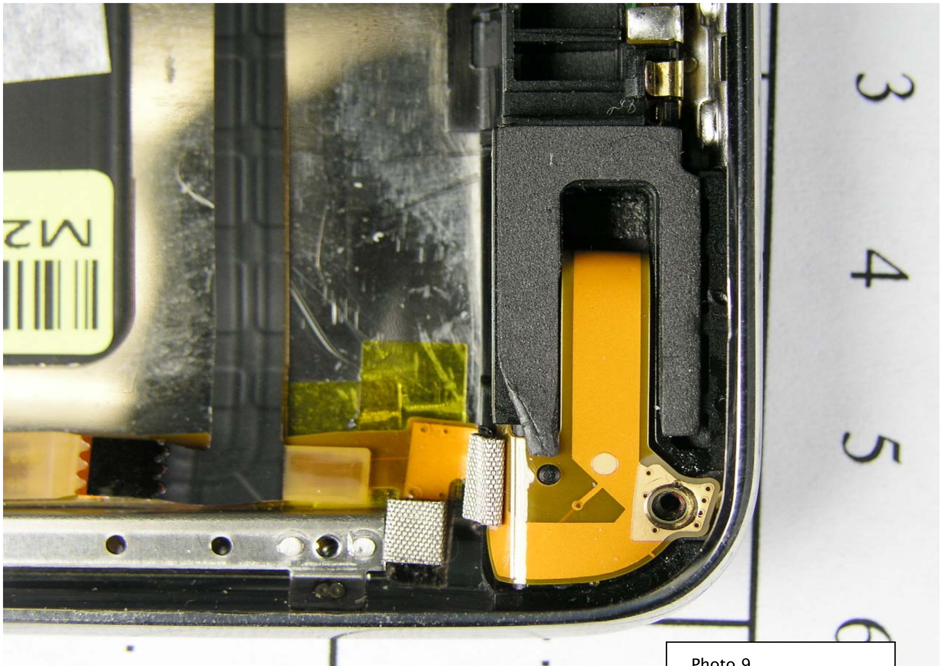
Photo 9 A1318, Antenna flex cable
