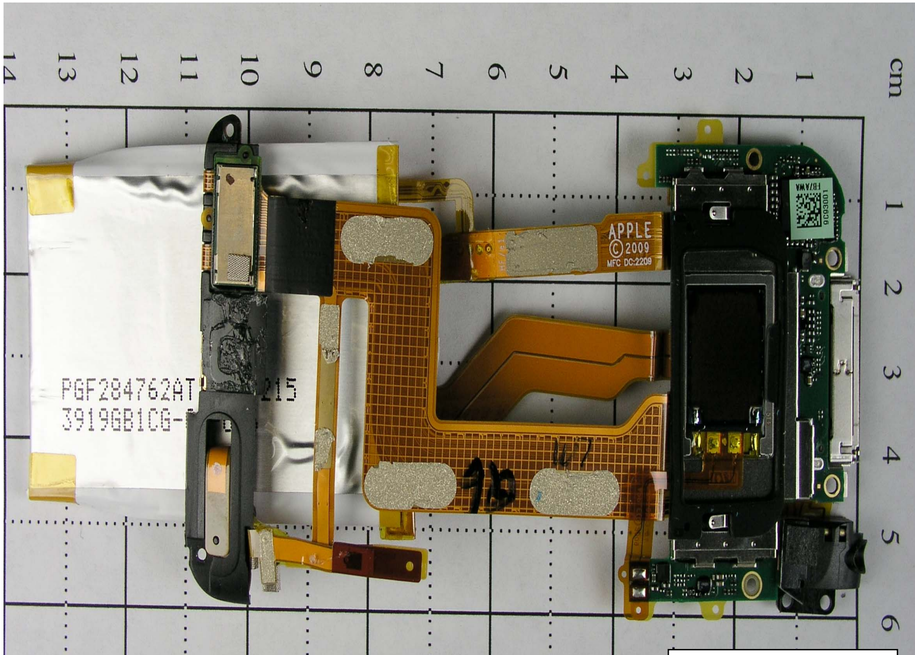
Photo 10 A1318. iPod PCB, Flex Cable WiFi Module board
