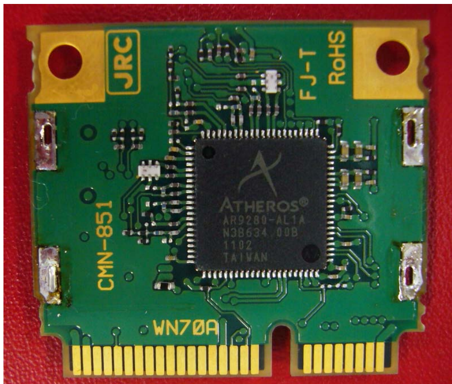
WLAN Circuit (Bottom) without Shield
