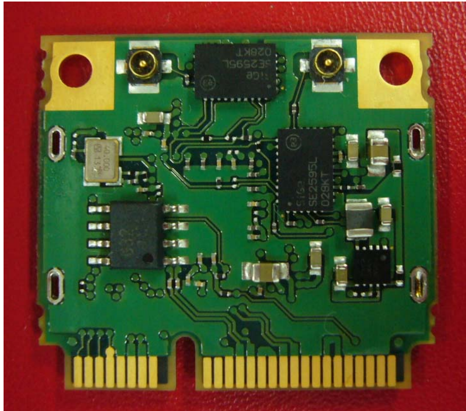
WLAN Circuit (Top) without Shield
