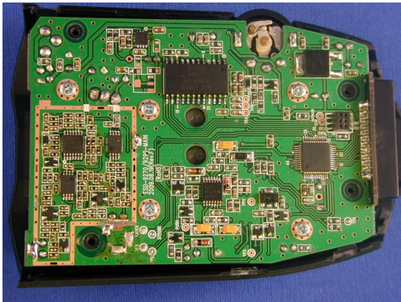
MODEL ESD9290 – MAIN PCB BOTTOM VIEW - NS
