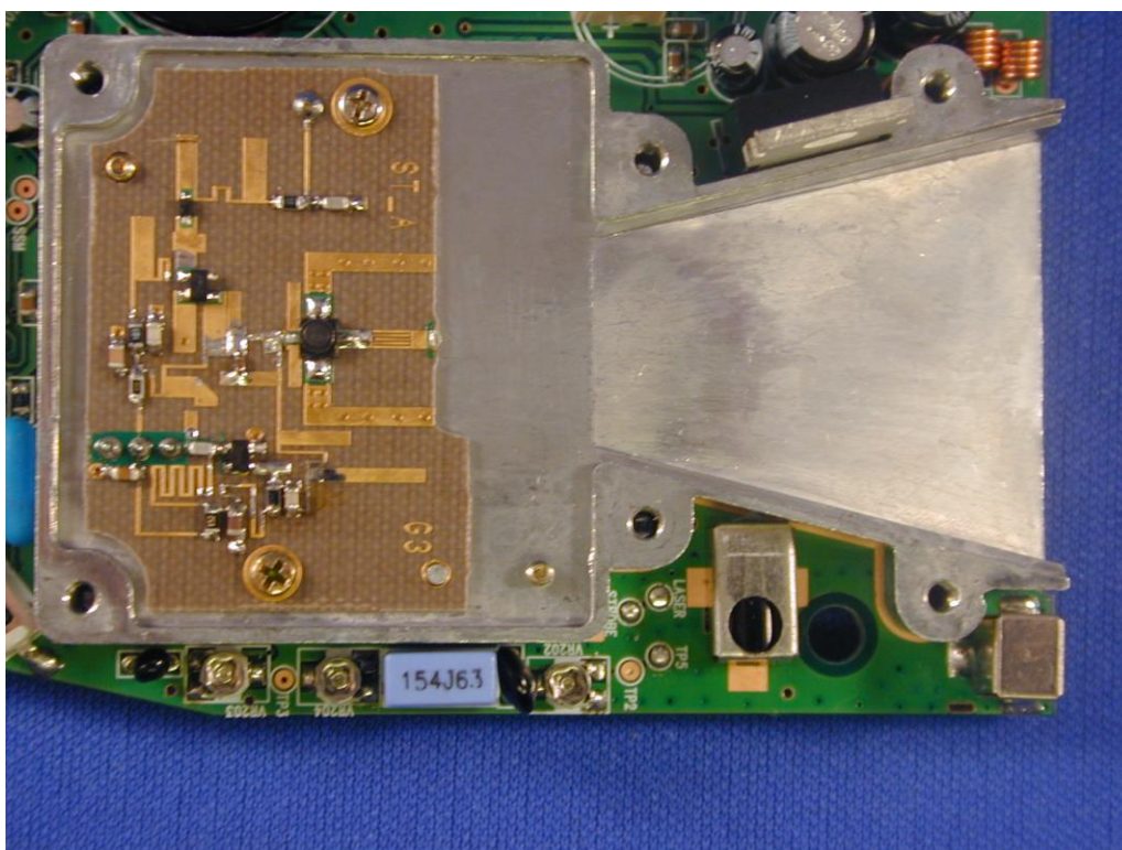
MODEL ESD9270 AND ESD9290 LNA PCB TOP VIEW
