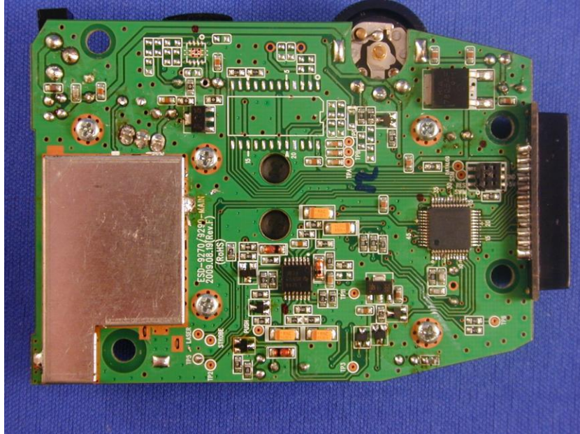
MODEL ESD9290 MAIN PCB BOTTOM VIEW WITH SHIELD
