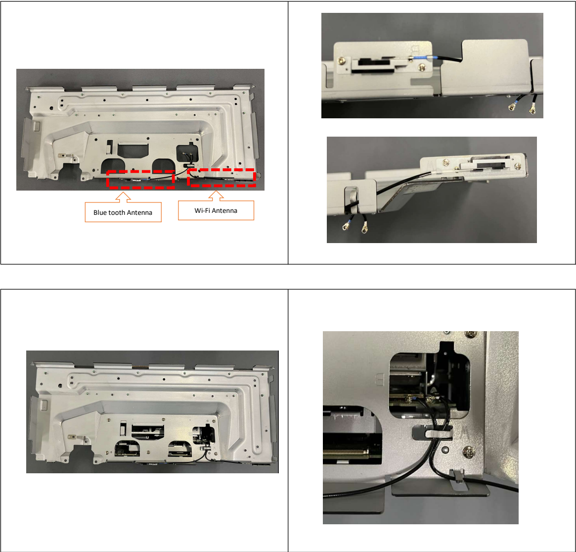
Internal view
