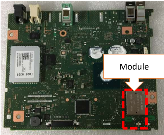
Component side
