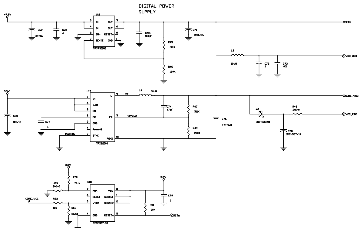
RESET CIRCUIT
