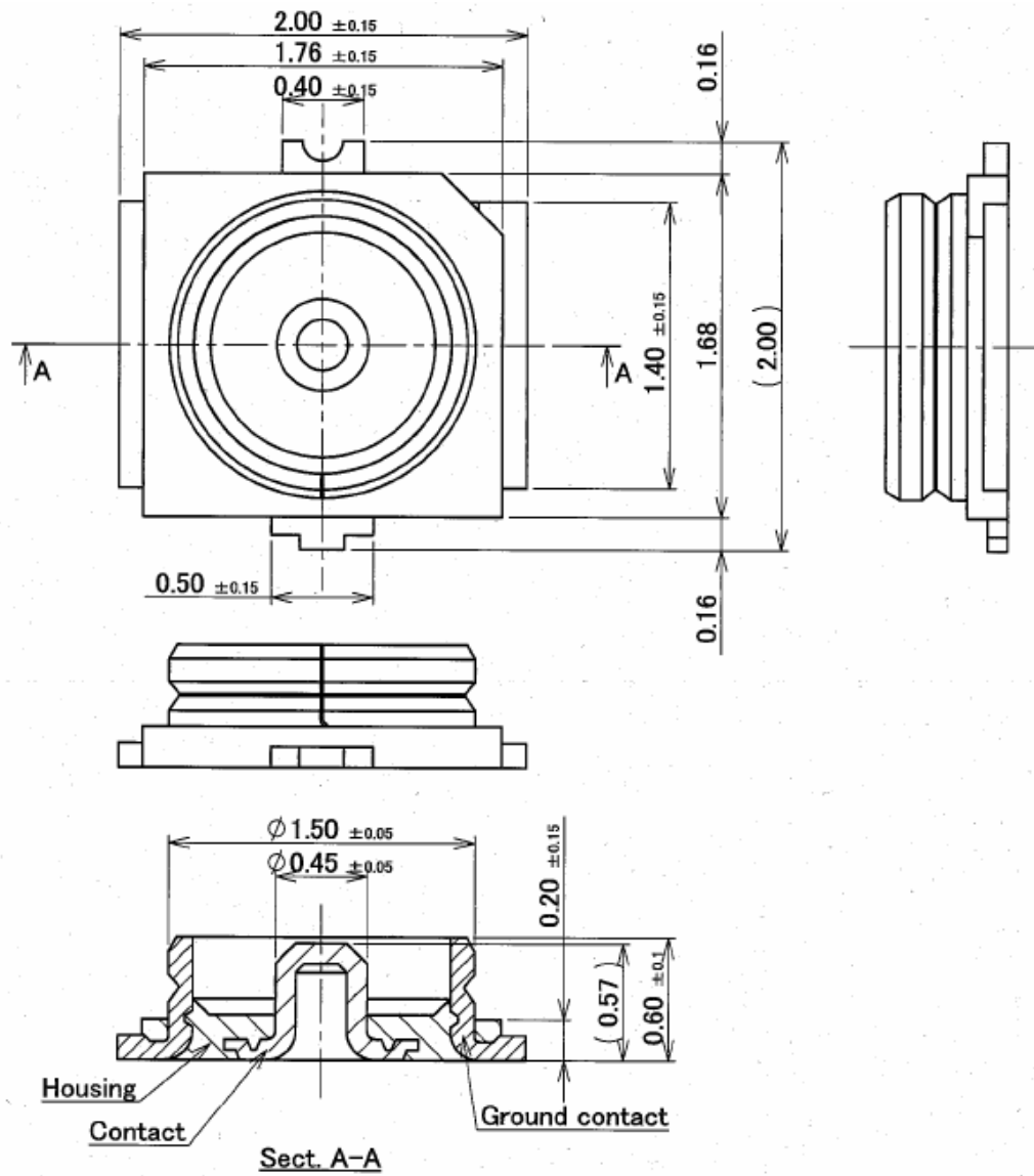
Figure 2-2 RF connectors
