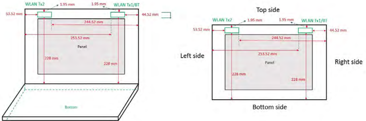
Photograph 17. Antenna position of EUT
