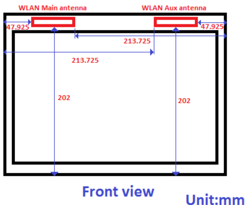
Fig.10 Antenna location of EUT (tablet mode)
