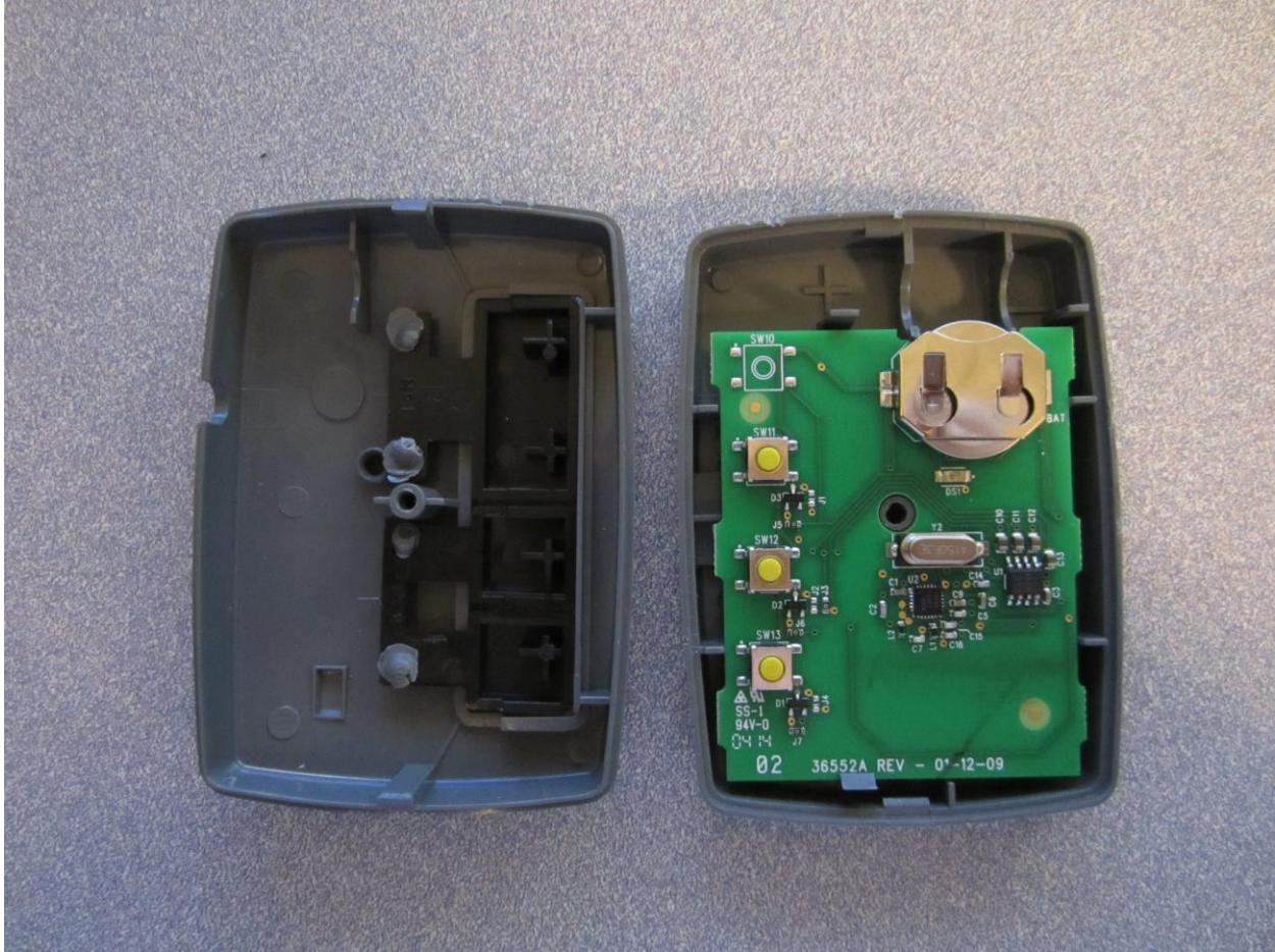
Figure 3: OCDFX5 Internal View / PCB Top
