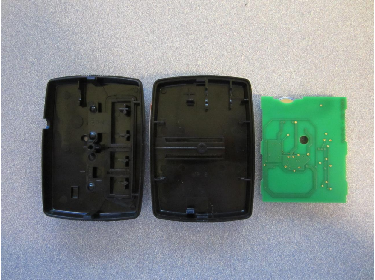
Figure 2: GIDFX5 Internal View / PCB Bottom
