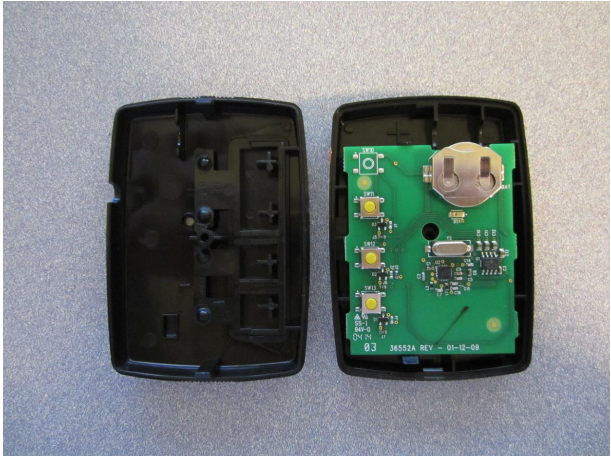
Figure 1: GIDFX5 Internal View / PCB Top
