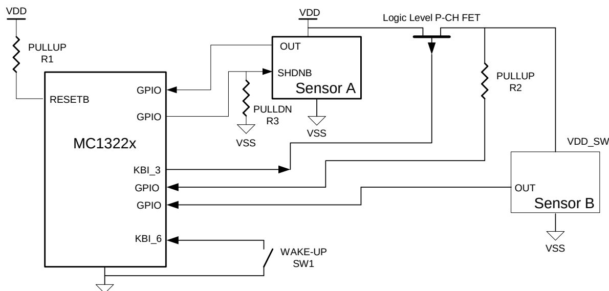
Figure 3-5. MC1322x as a Primary Device
