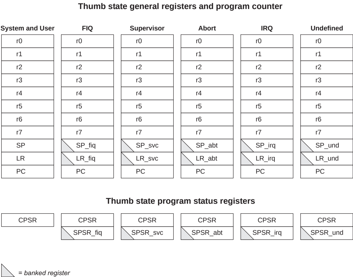
Figure 7-5. Register organization in Thumb state
