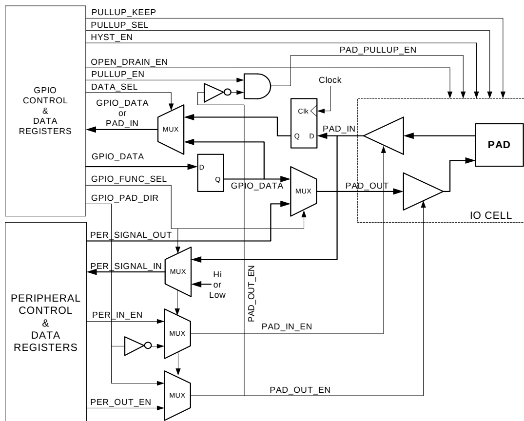
Figure 11-1. GPIO Typical Single-Bit Block Diagram.
