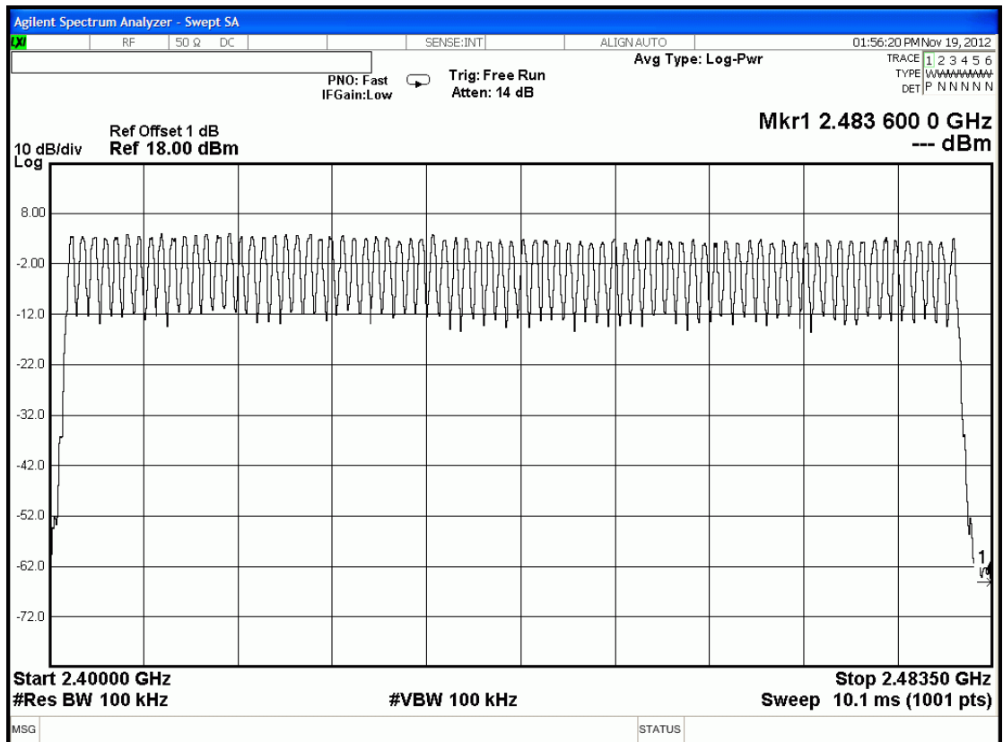
Figure 2: GFSK
