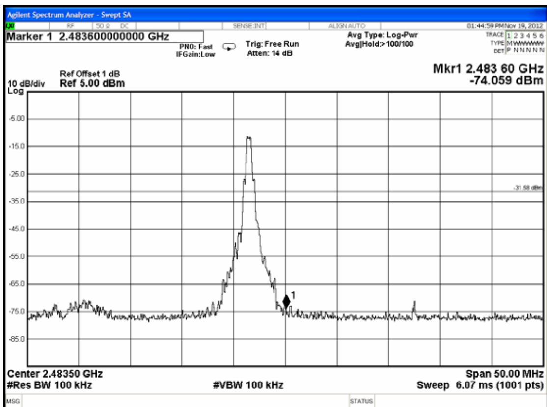
Figure 6: GFSK, Upper Band edge
