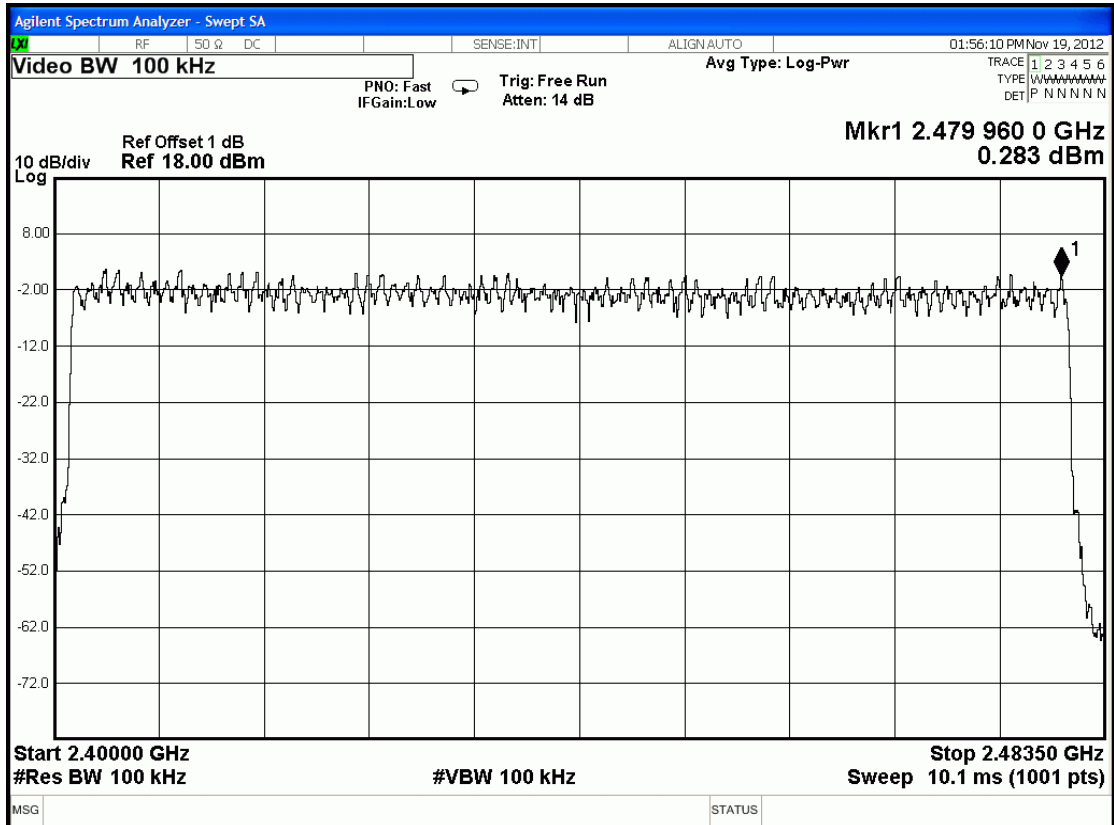
Figure 1: 8-DPSK
