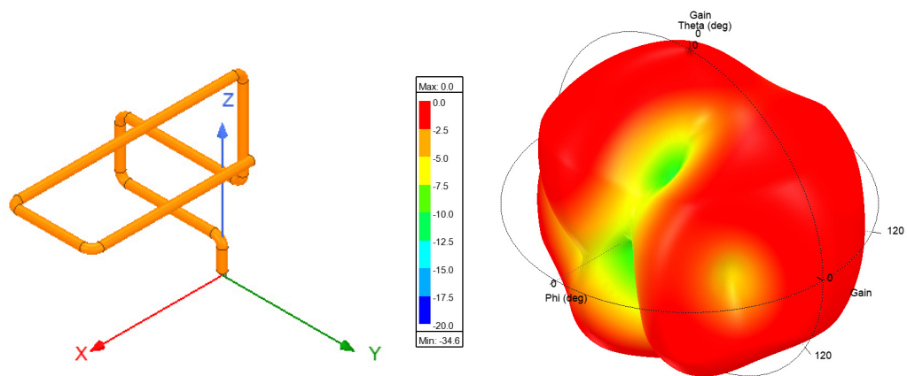
Radiation Pattern
