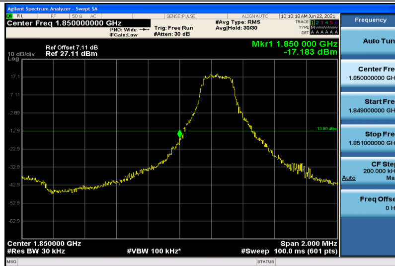
Band25-3MHz-QPSK-26055-1RB#0
