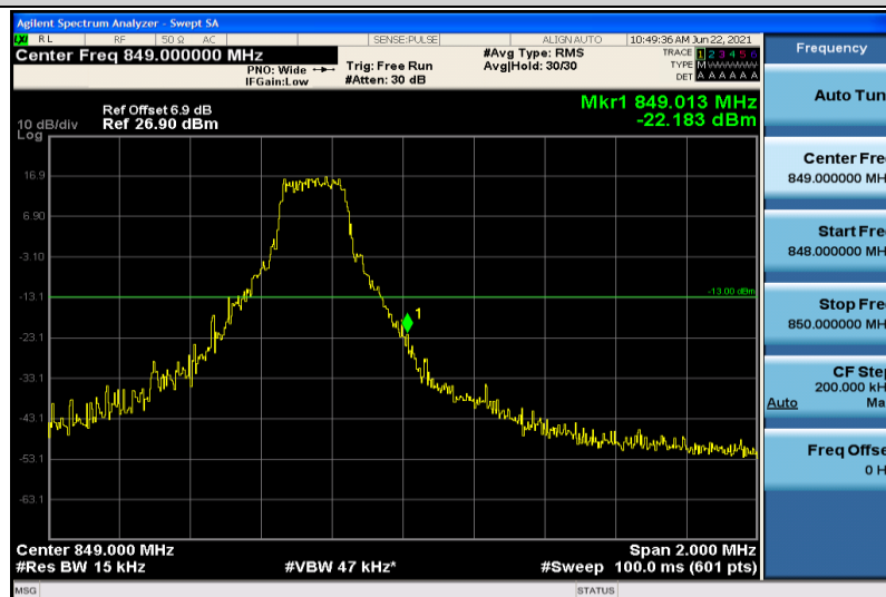
Band26-1.4MHz-QPSK-27033-1RB#5
