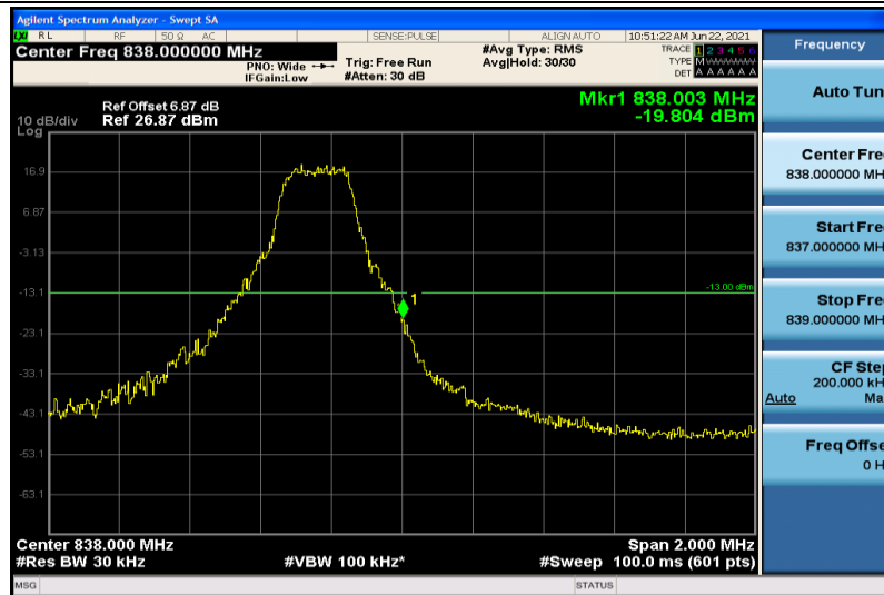
Band26-3MHz-QPSK-26915-1RB#14
