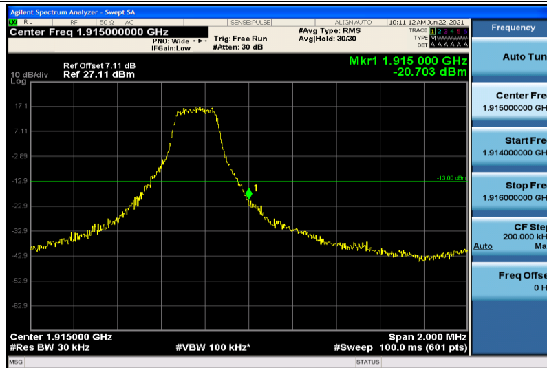
Band25-3MHz-16QAM-26675-1RB#14
