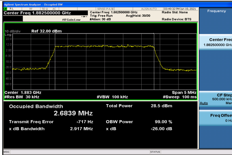
Band25-3MHz-16QAM-26365-15RB#0-2.6839
