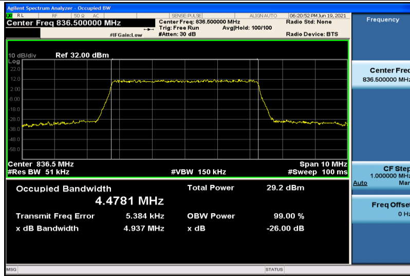
Band26-5MHz-16QAM-26915-25RB#0-4.4781
