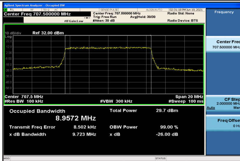
Band12-10MHz-16QAM-23095-50RB#0-8.9572
