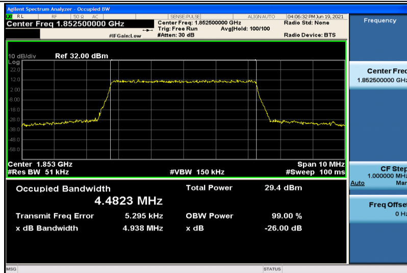
Band25-5MHz-16QAM-26065-25RB#0-4.4823
