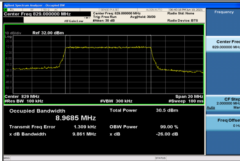
Band26-10MHz-QPSK-26840-50RB#0-8.9685
