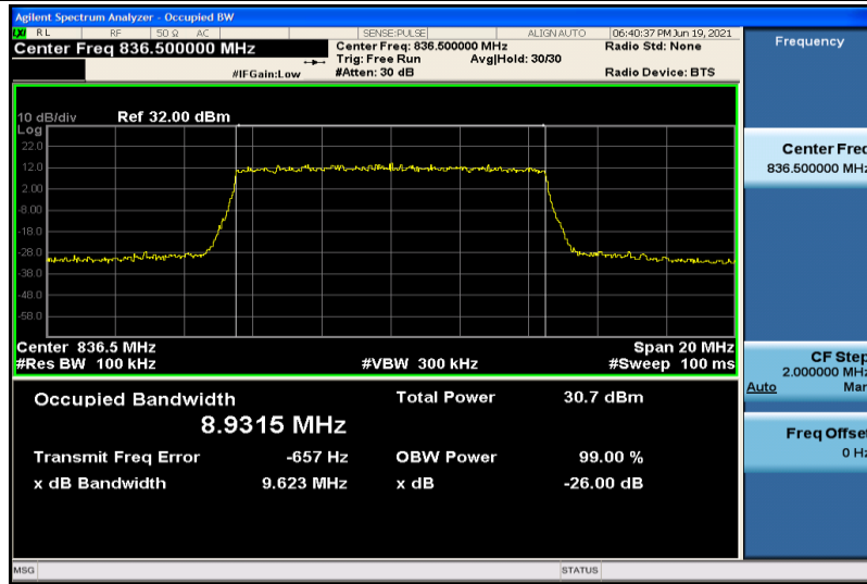
Band26-10MHz-QPSK-26915-50RB#0-8.9315
