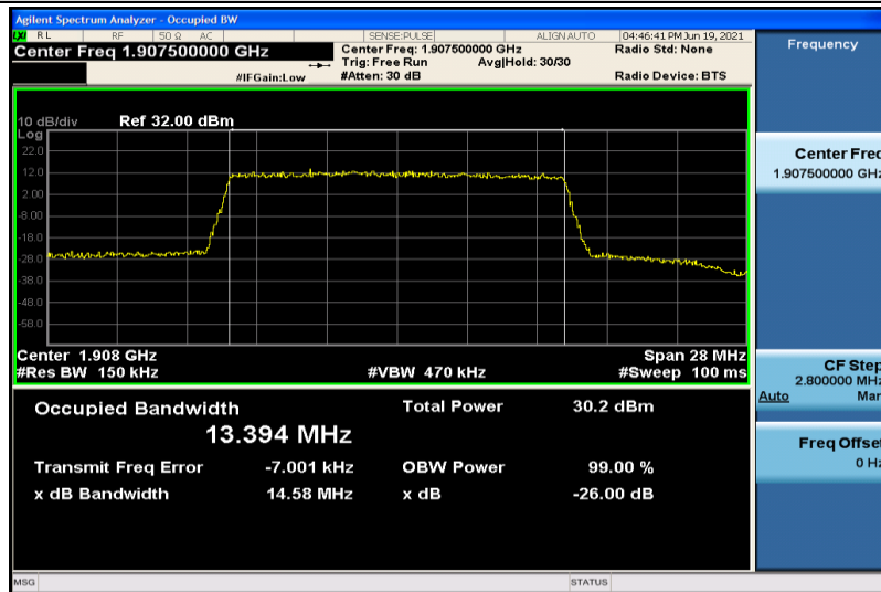
Band25-15MHz-QPSK-26615-75RB#0-13.394
