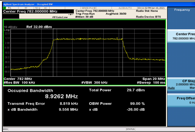
Band13-10MHz-16QAM-23230-50RB#0-8.9262
