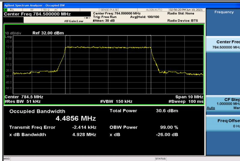
Band13-5MHz-QPSK-23255-25RB#0-4.4856
