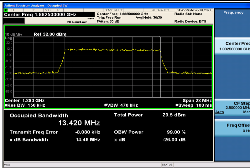
Band25-15MHz-16QAM-26365-75RB#0-13.420
