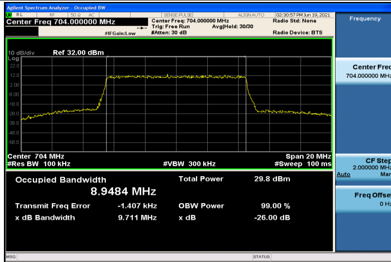
Band12-10MHz-16QAM-23060-50RB#0-8.9484
