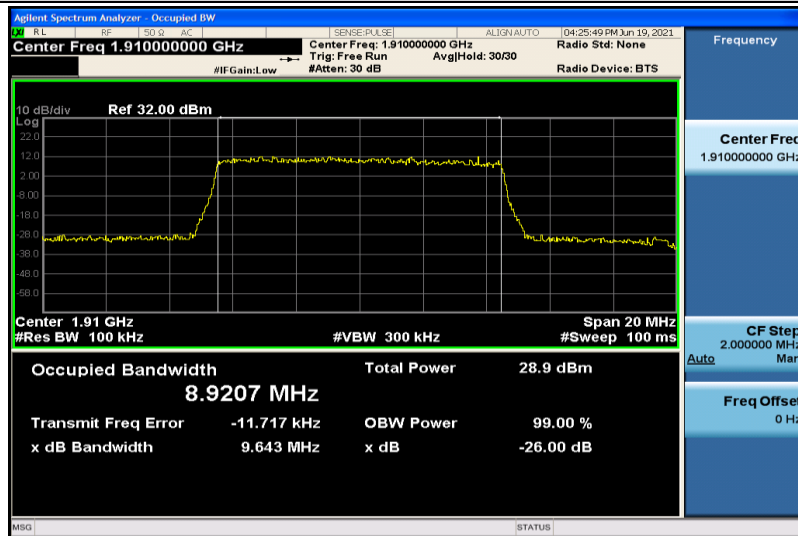
Band25-10MHz-16QAM-26640-50RB#0-8.9207
