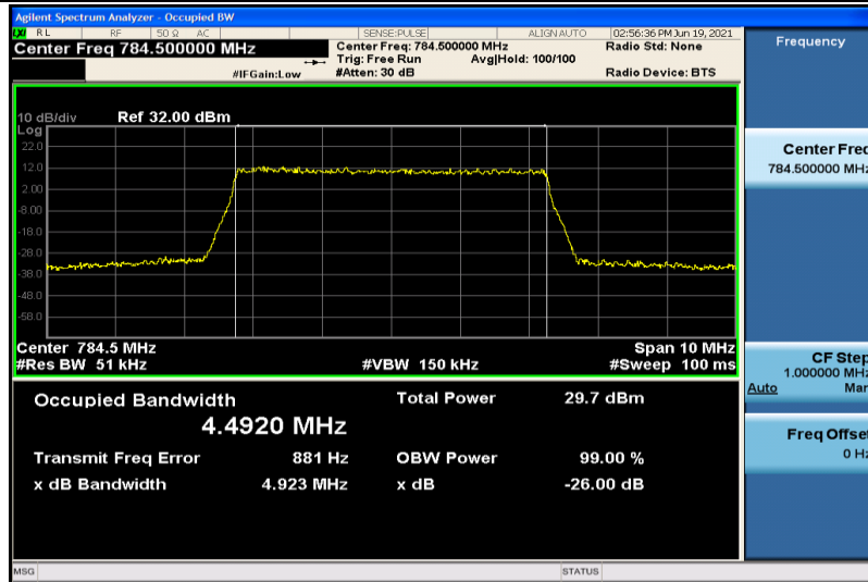
Band13-5MHz-16QAM-23255-25RB#0-4.4920
