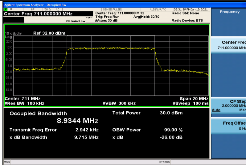
Band12-10MHz-16QAM-23130-50RB#0-8.9344
