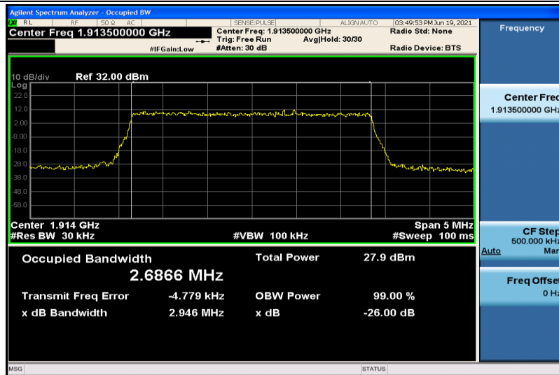
Band25-3MHz-16QAM-26675-15RB#0-2.6866
