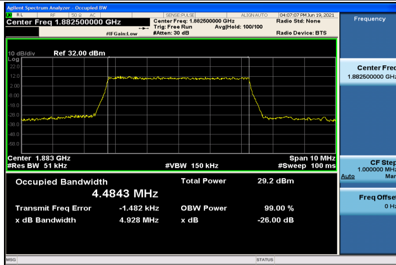
Band25-5MHz-16QAM-26365-25RB#0-4.4843
