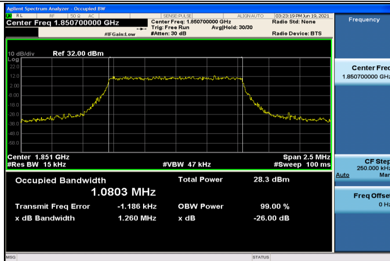
Band25-1.4MHz-16QAM-26047-6RB#0-1.0803
