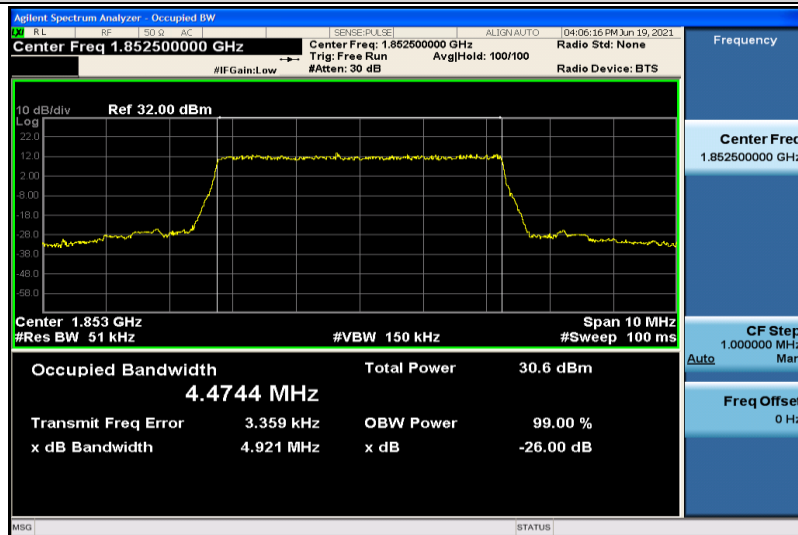
Band25-5MHz-QPSK-26065-25RB#0-4.4744
