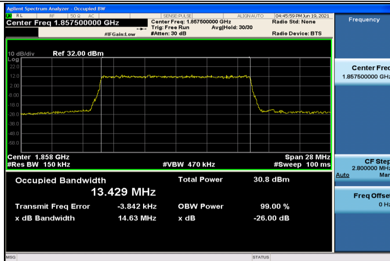
Band25-15MHz-QPSK-26115-75RB#0-13.429
