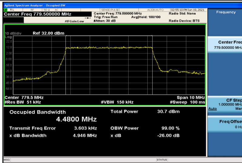
Band13-5MHz-QPSK-23205-25RB#0-4.4800
