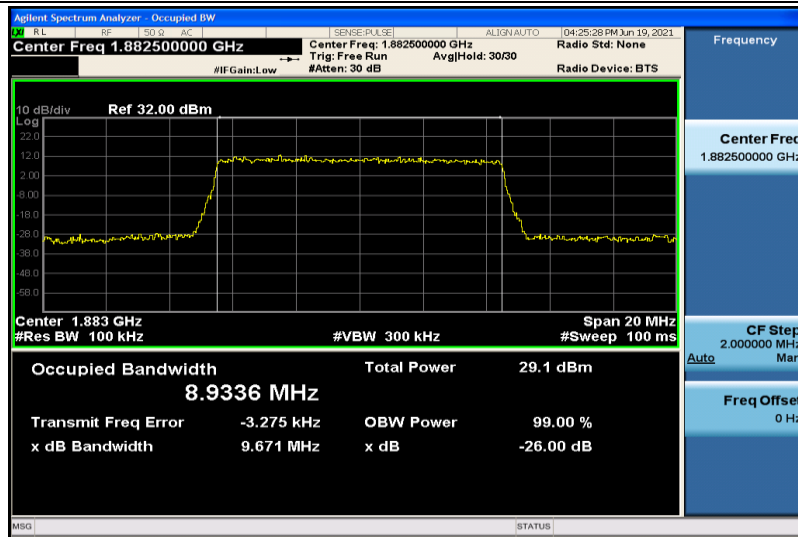
Band25-10MHz-16QAM-26365-50RB#0-8.9336
