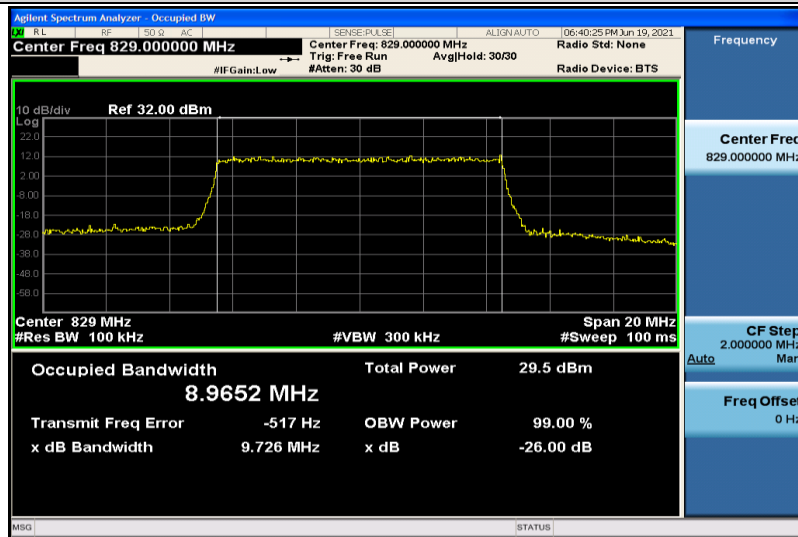
Band26-10MHz-16QAM-26840-50RB#0-8.9652
