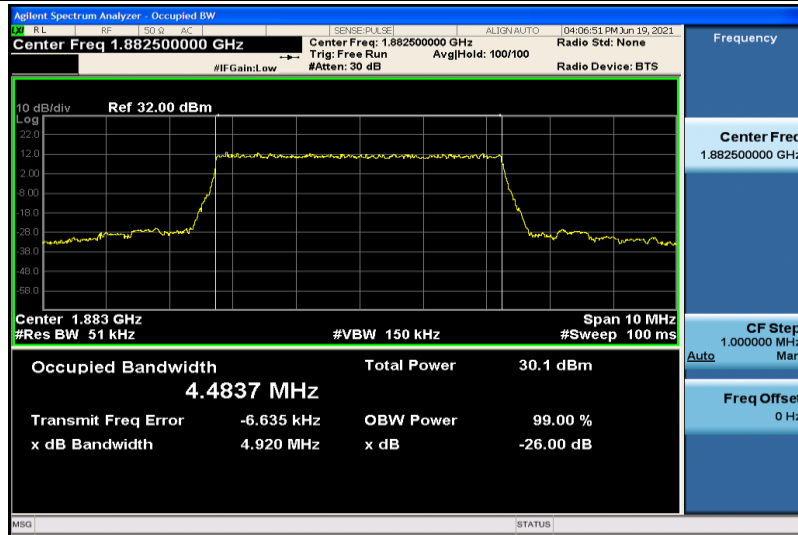
Band25-5MHz-QPSK-26365-25RB#0-4.4837
