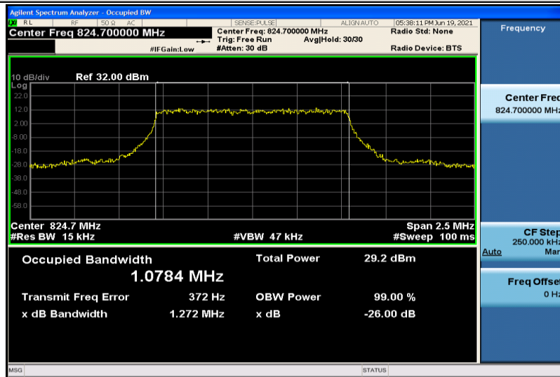
Band26-1.4MHz-QPSK-26797-6RB#0-1.0784
