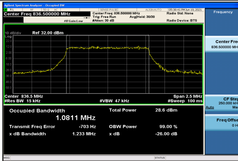
Band26-1.4MHz-16QAM-26915-6RB#0-1.0811
