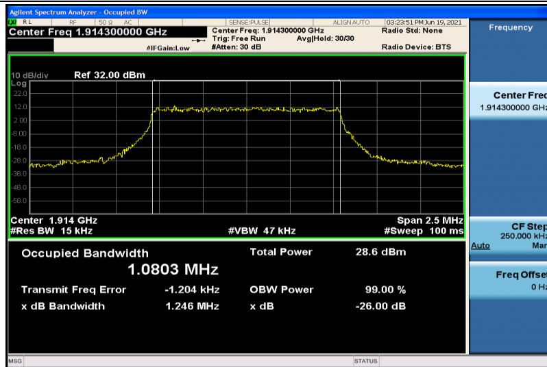
Band25-1.4MHz-QPSK-26683-6RB#0-1.0803
