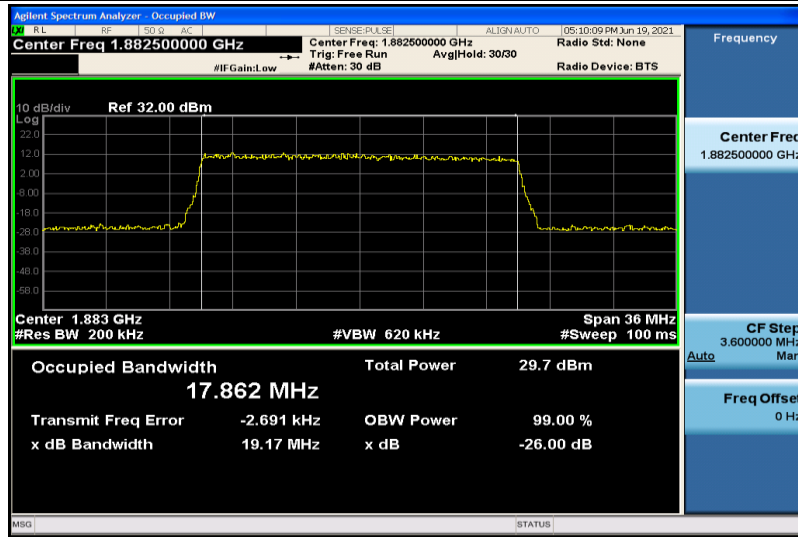
Band25-20MHz-16QAM-26365-100RB#0-17.862
