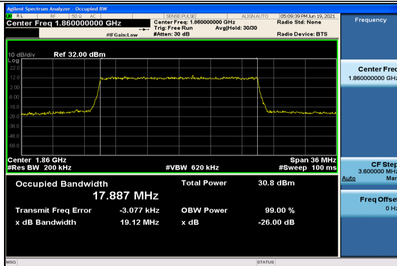
Band25-20MHz-QPSK-26140-100RB#0-17.887
