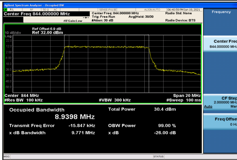
Band26-10MHz-QPSK-26990-50RB#0-8.9398
