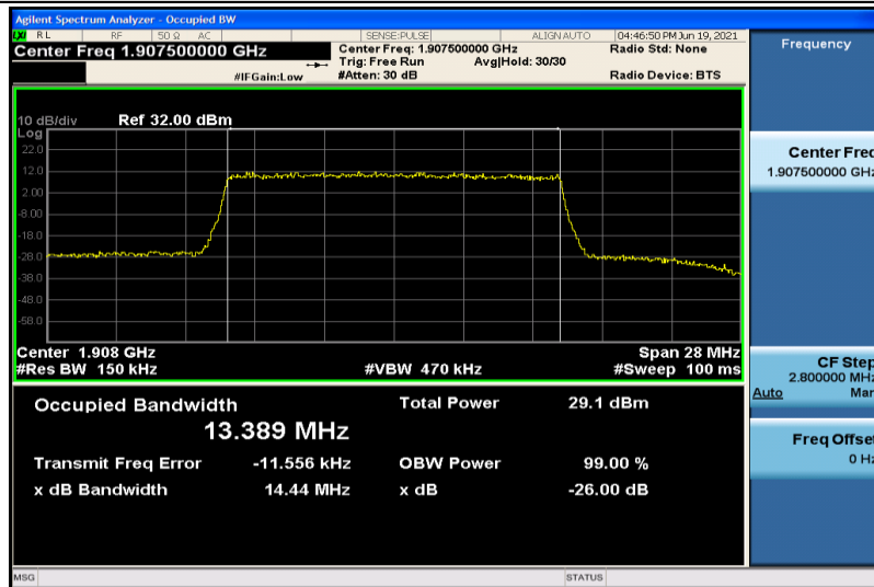
Band25-15MHz-16QAM-26615-75RB#0-13.389
