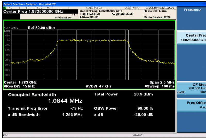
Band25-1.4MHz-QPSK-26365-6RB#0-1.0844
