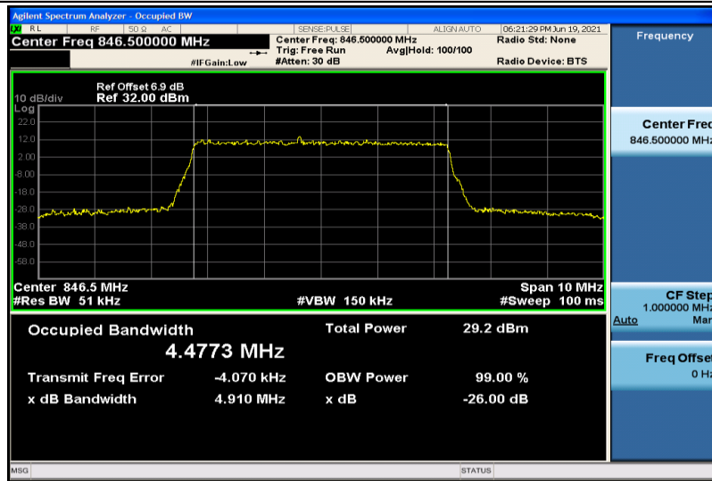
Band26-5MHz-16QAM-27015-25RB#0-4.4773
