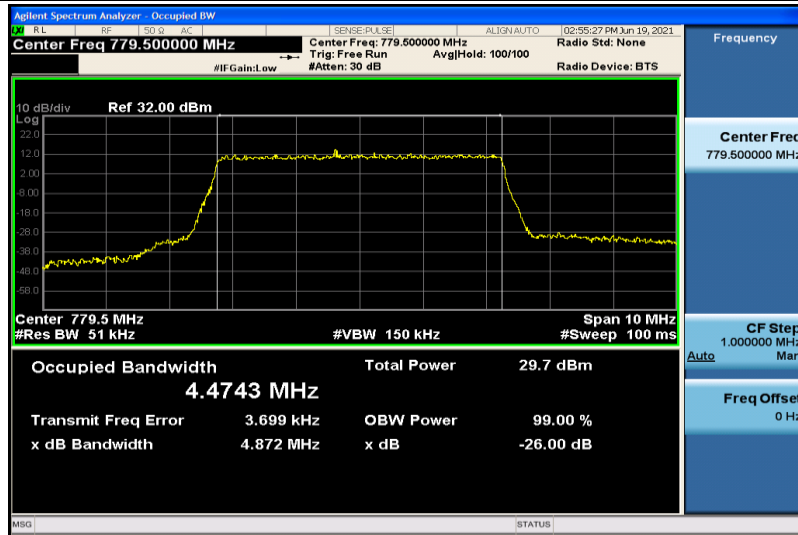
Band13-5MHz-16QAM-23205-25RB#0-4.4743
