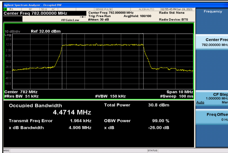
Band13-5MHz-QPSK-23230-25RB#0-4.4714
