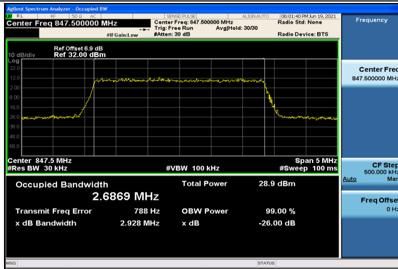
Band26-3MHz-16QAM-27025-15RB#0-2.6869
