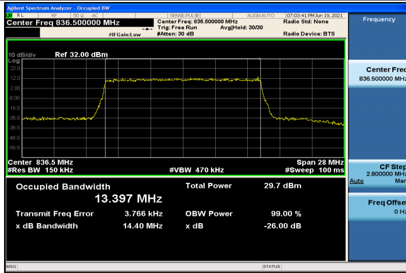
Band26-15MHz-16QAM-26915-75RB#0-13.397
