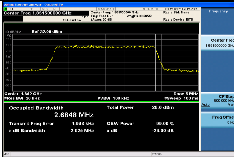
Band25-3MHz-16QAM-26055-15RB#0-2.6848
