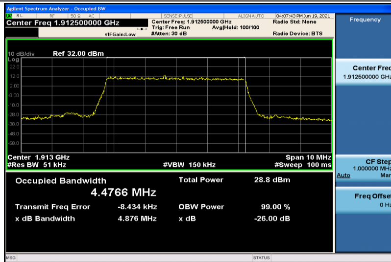
Band25-5MHz-16QAM-26665-25RB#0-4.4766
