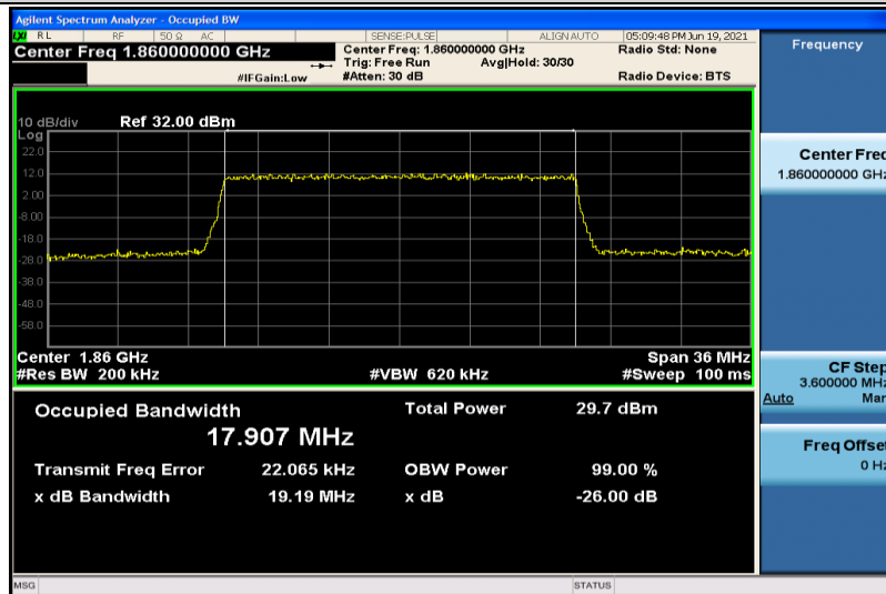
Band25-20MHz-16QAM-26140-100RB#0-17.907
