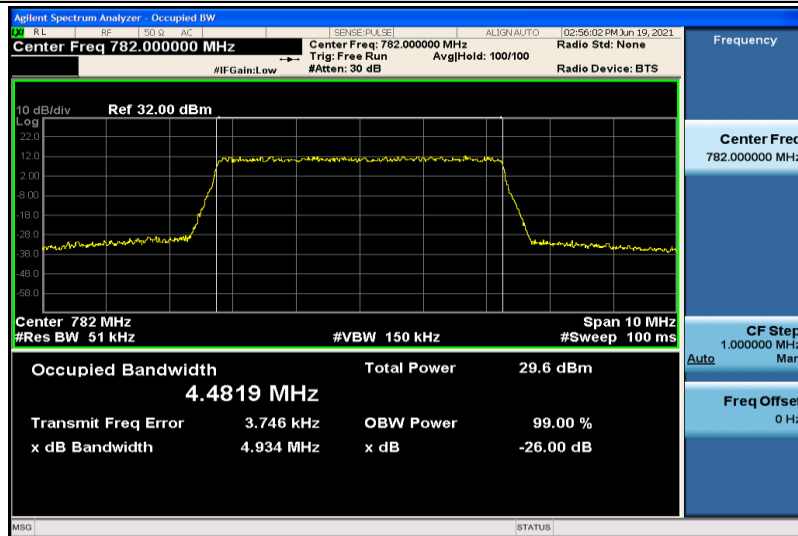
Band13-5MHz-16QAM-23230-25RB#0-4.4819
