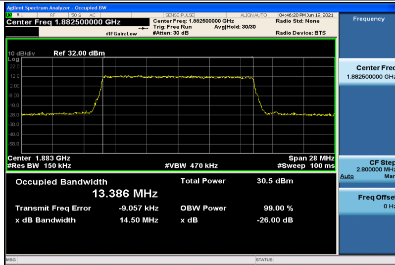
Band25-15MHz-QPSK-26365-75RB#0-13.386
