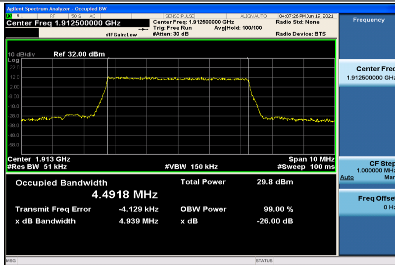
Band25-5MHz-QPSK-26665-25RB#0-4.4918
