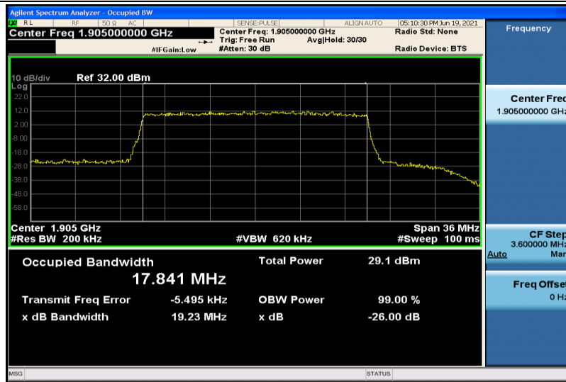
Band25-20MHz-16QAM-26590-100RB#0-17.841
