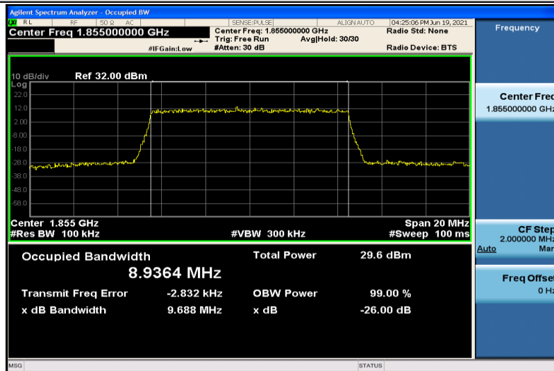
Band25-10MHz-16QAM-26090-50RB#0-8.9364
