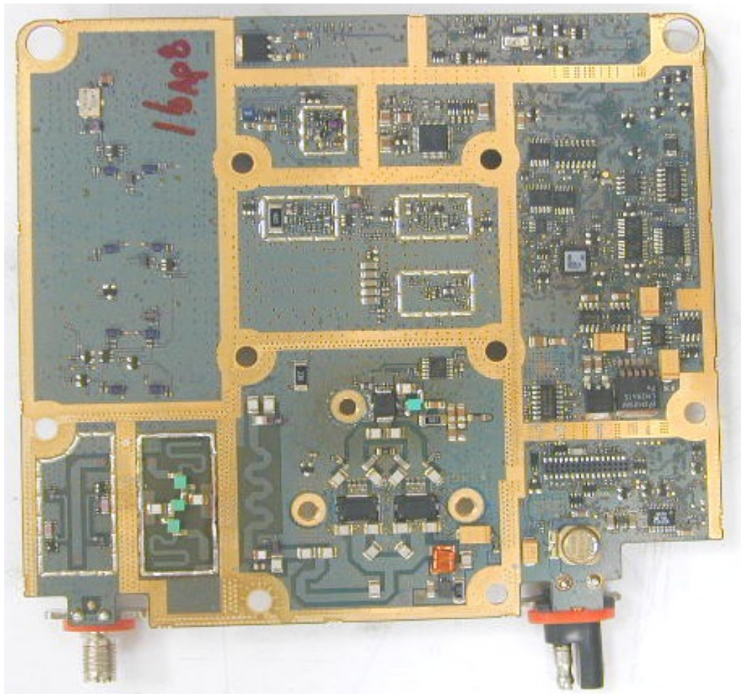
RADIO BOARD, less shields (TOP VIEW)
