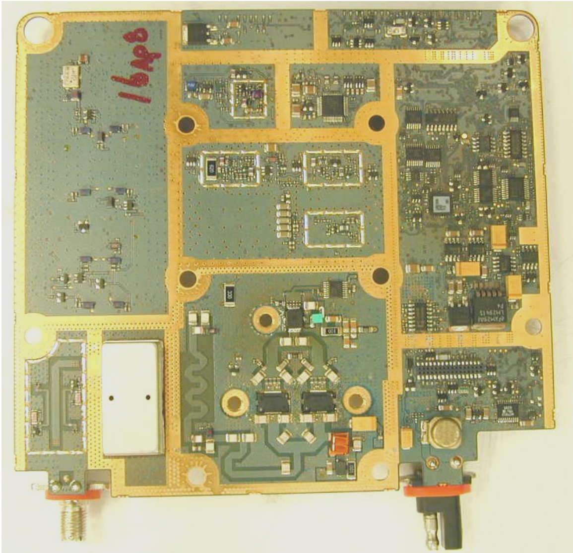
RADIO BOARD (TOP VIEW)
