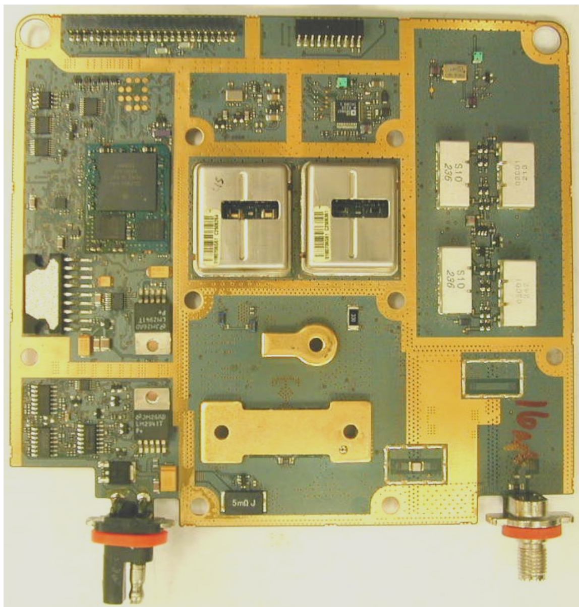
RADIO BOARD (BOTTOM VIEW)
