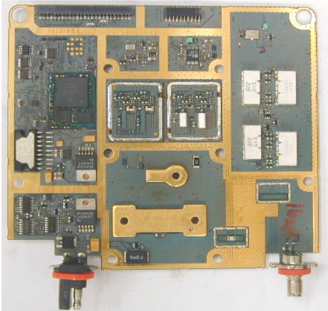
RADIO BOARD, less shields (BOTTOM VIEW)
