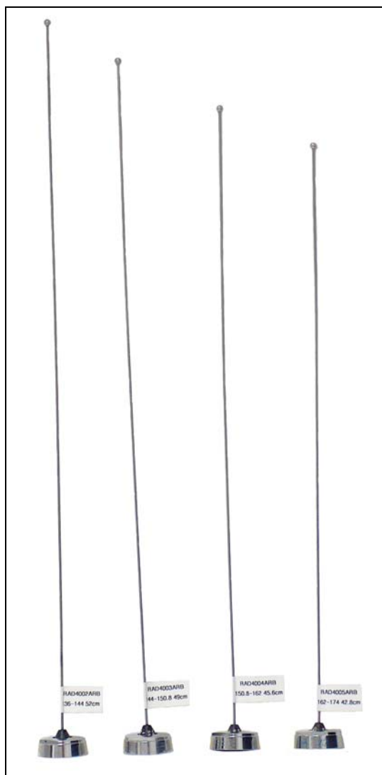
Antenna kit numbers, from left to right; RAD4002ARB (136MHz), RAD4003ARB (147.4MHz), RAD4004ARB (155MHz), RAD4005ARB (174MHz),
