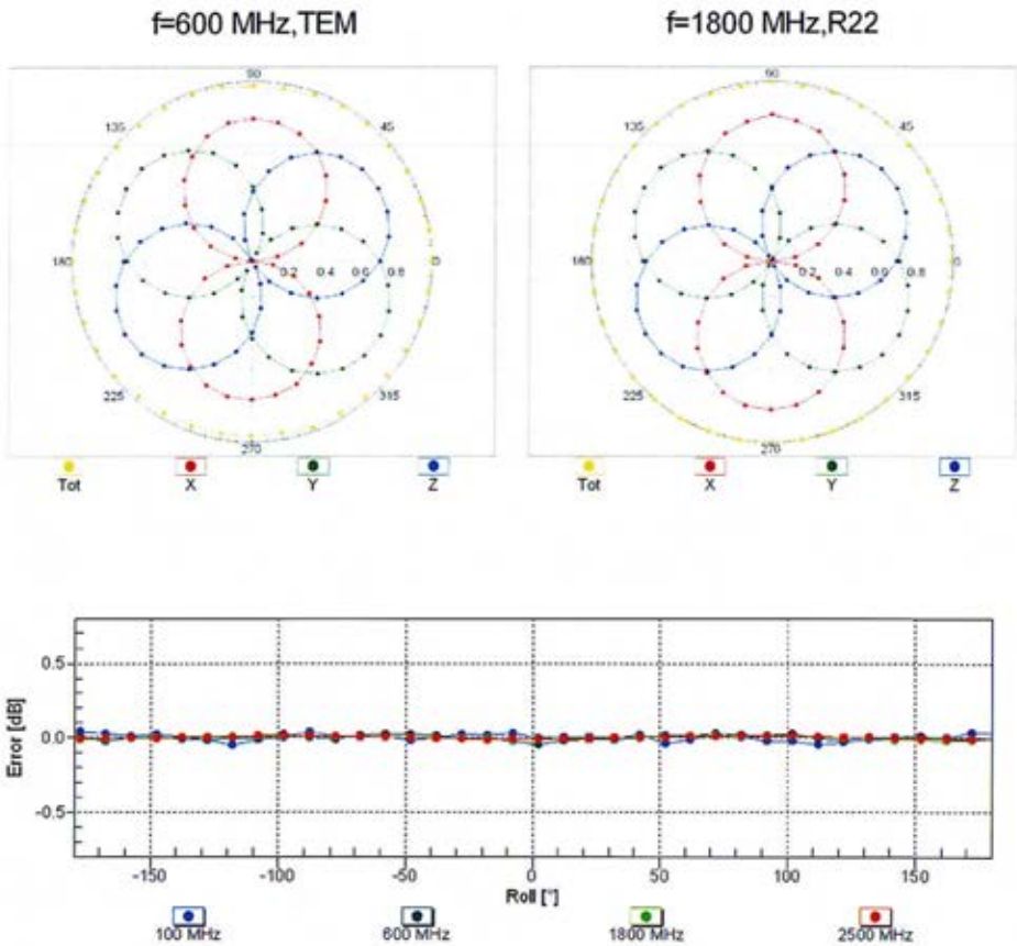
Uncertainty of Axial Isotropy Assessment: \pm 0.5\% ( k=2 )
