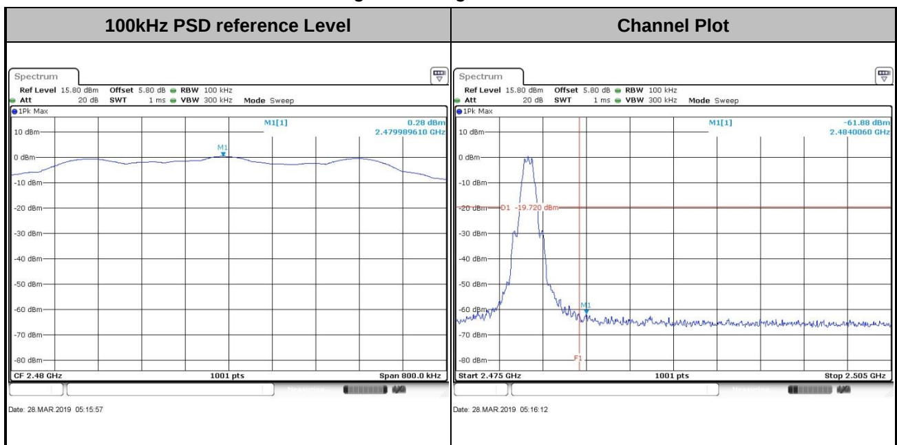
High Band Edge Plot on Channel 39
