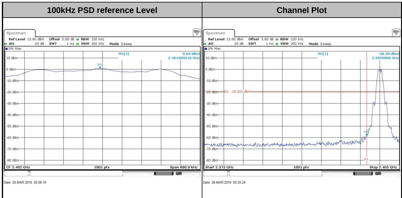
Low Band Edge Plot on Channel 00
