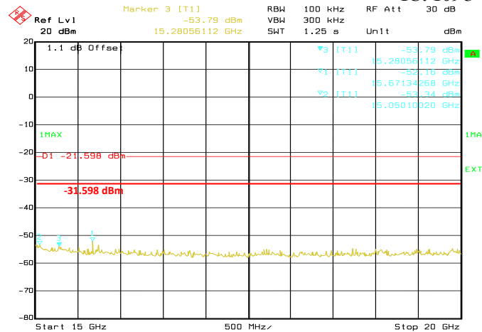
Conducted Emissions. 802.11n, Frequency 2437 MHz Emission Level, 15 GHz -> 20 GHz
