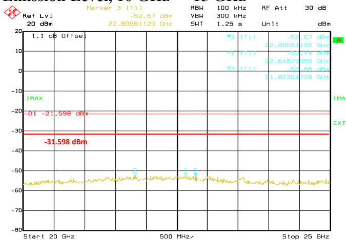
Conducted Emissions. 802.11n, Frequency 2437 MHz Emission Level, 20 GHz -> 25 GHz
