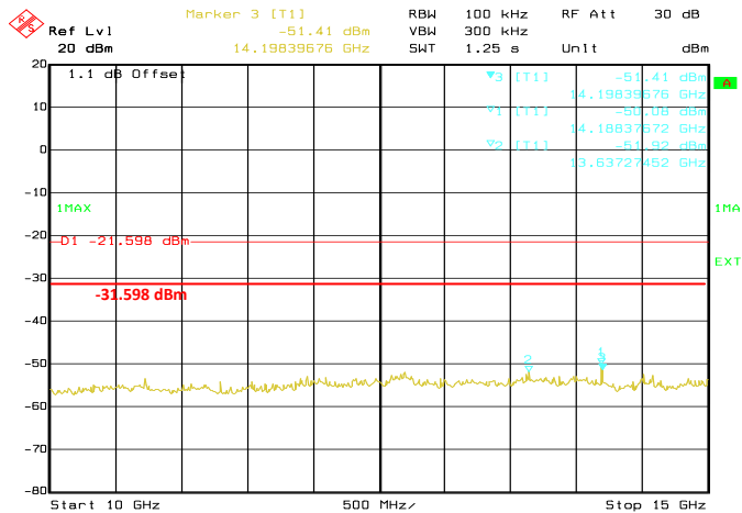
Conducted Emissions. 802.11n, Frequency 2437 MHz Emission Level, 10 GHz -> 15 GHz
