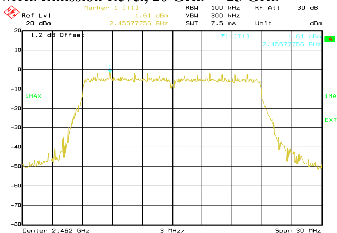
Conducted Emissions. 802.11n, Frequency 2462 MHz Reference Level
