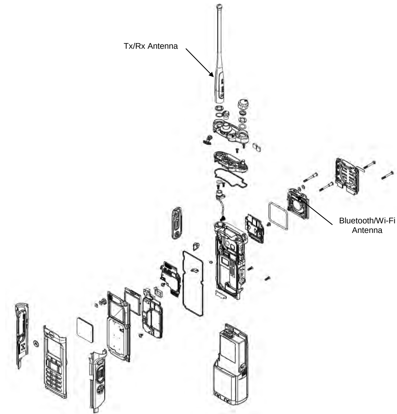
Exploded view of APX6000/APX6000Li/APX5000/SRX2200 Model 3.5
