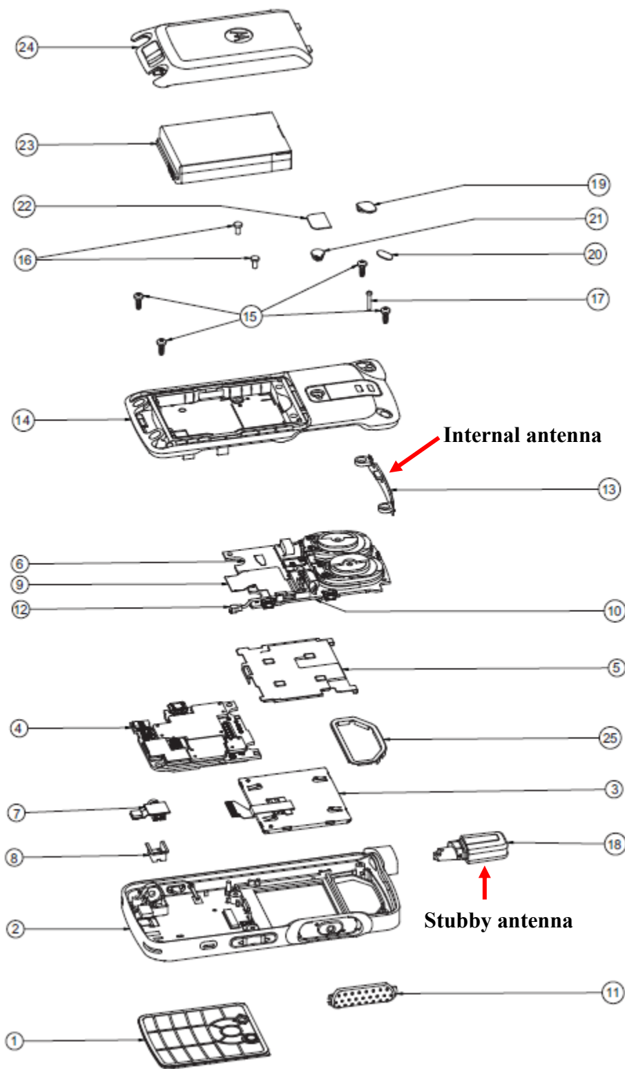
Exploded View of GOB Model
