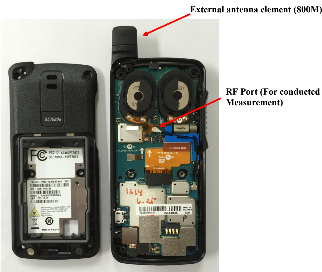
PCB board with housing (Back)
