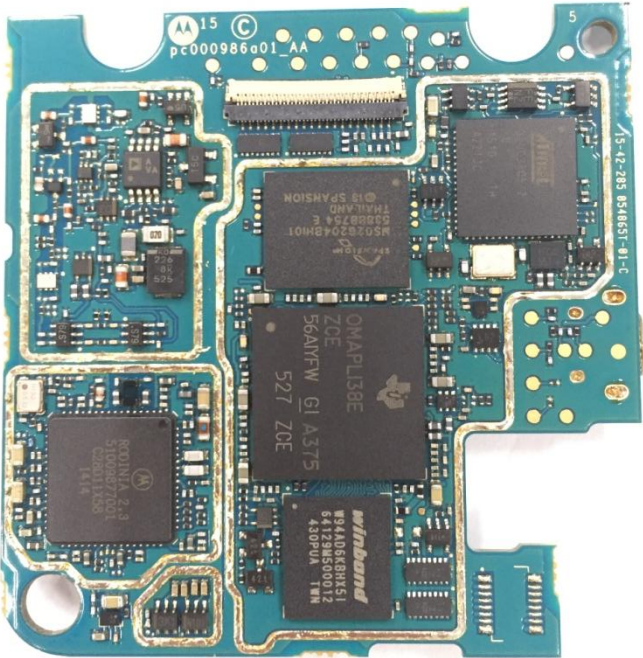
RF board without Shields (Top)
