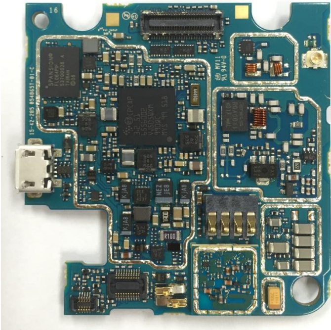
RF board without Shields (Bottom)
