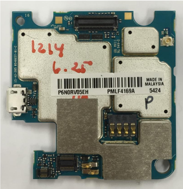
RF board with Shields (Bottom)
