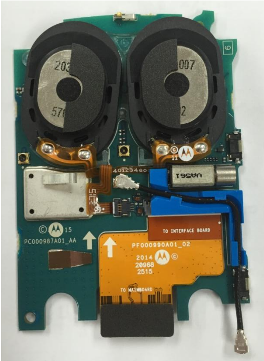
Interface board with Shields (Top)
