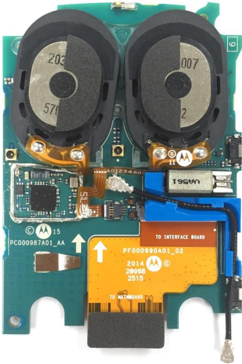
Interface board without shields (Top)
