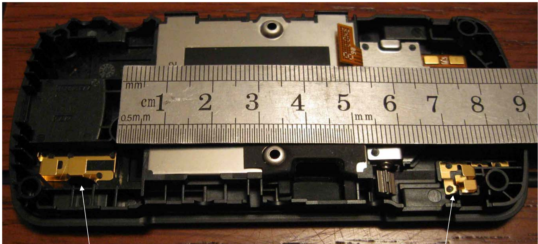
BT antenna on radio bottom side
