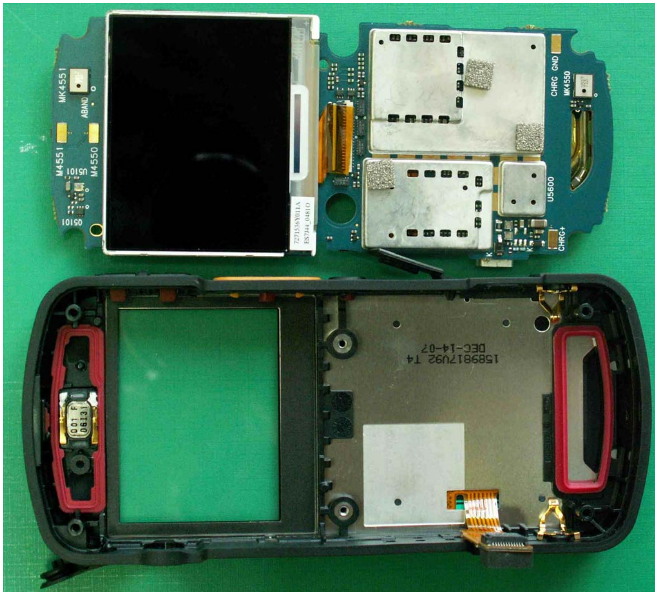
Photograph No. 1 F2978A Front housing and PCB front view
