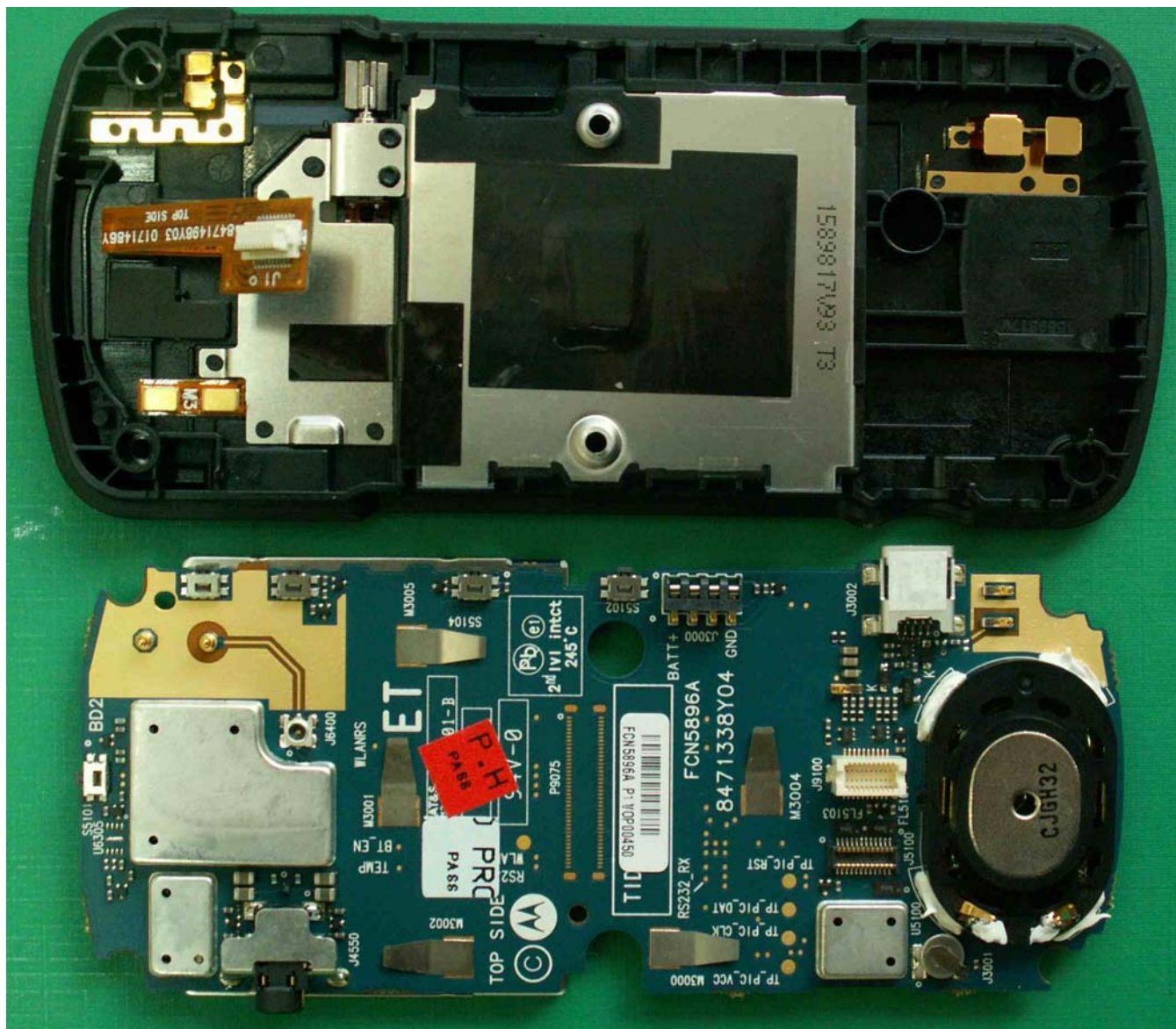
Photograph No. 2 F2978A Rear housing and PCB rear view
