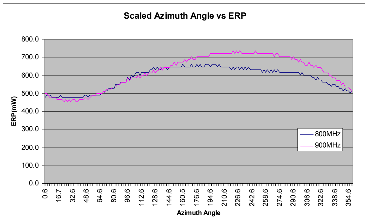
Figure 6-37: Scaled ERP vs. Azimuth Angle
