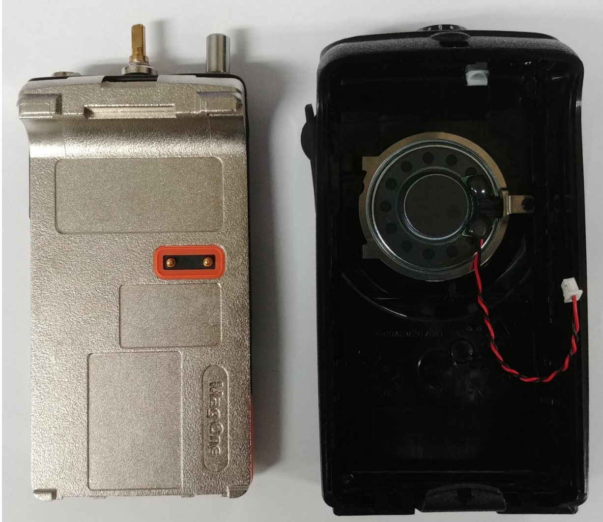
EXHIBIT 9E - Chassis and housing (Back Side)
