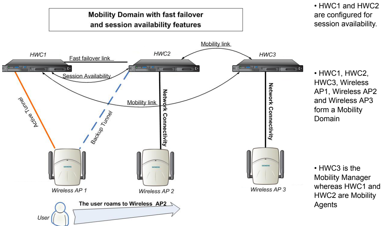
Figure 27 Mobility Domain with fast failover and session availability features
