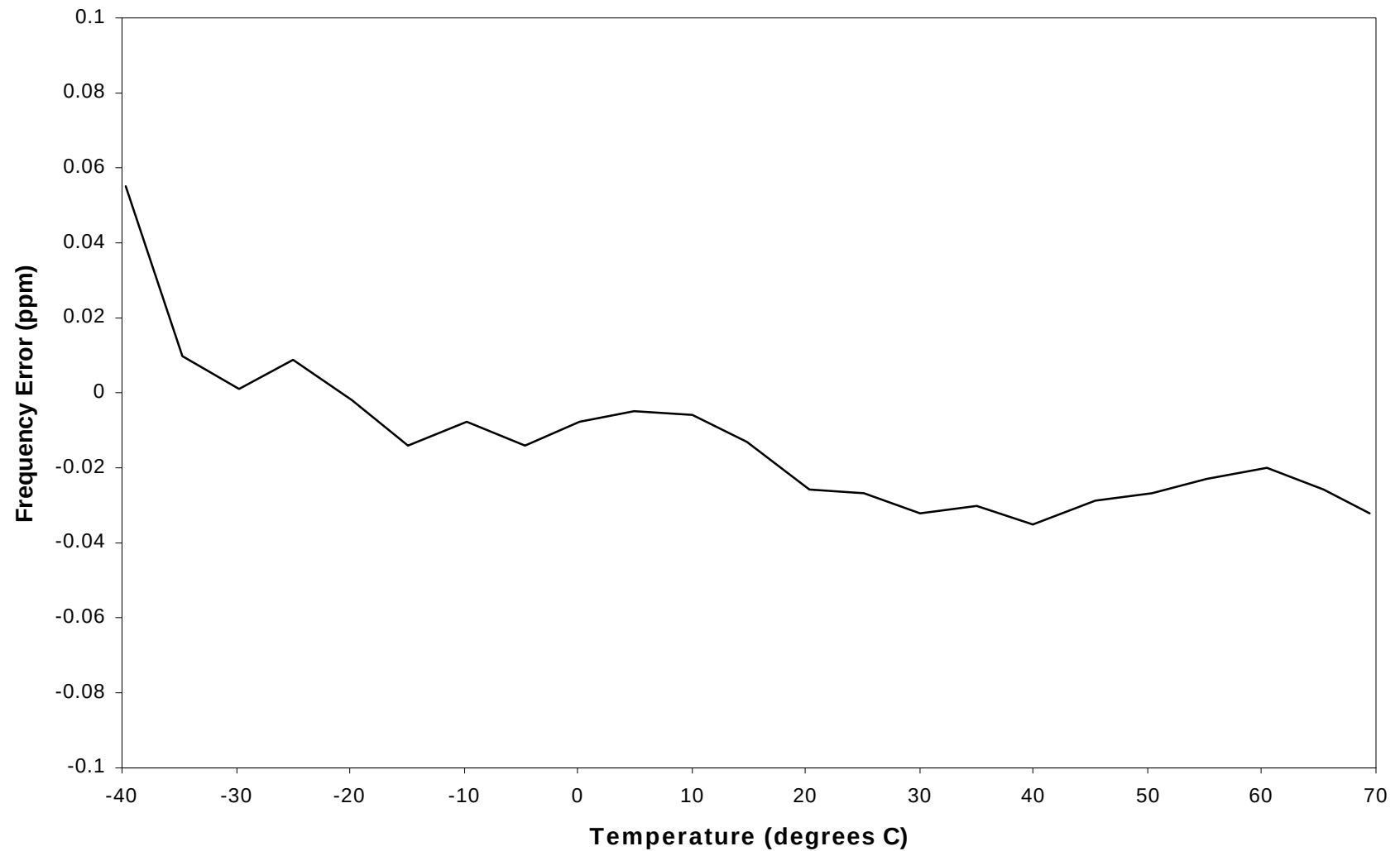
Exhibit 6F6: Frequency Stability versus Temperature, Digital Mode Voltage 6.0 VDC, Carrier Power +25.5 dBm, Frequency 835.02 MHz
