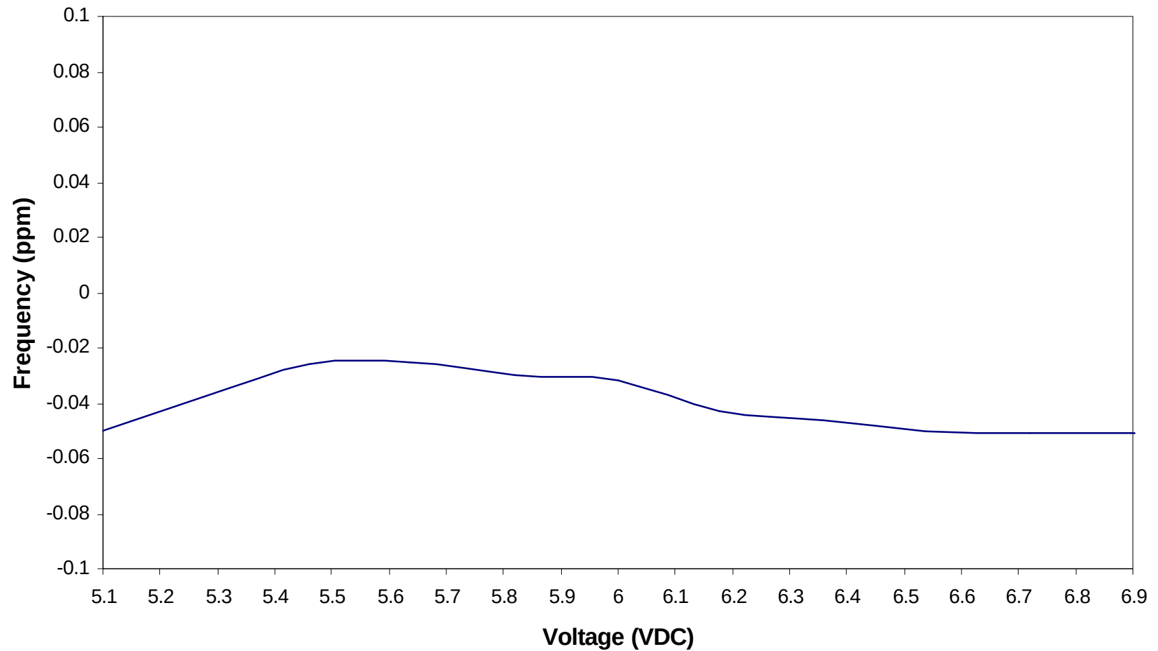
Exhibit 6F2: Transmitter Frequency Error versus Voltage, Analog Modulation Carrier Frequency 835.02 MHz, Carrier Power +35 dBm, Temperature 25 degrees C
