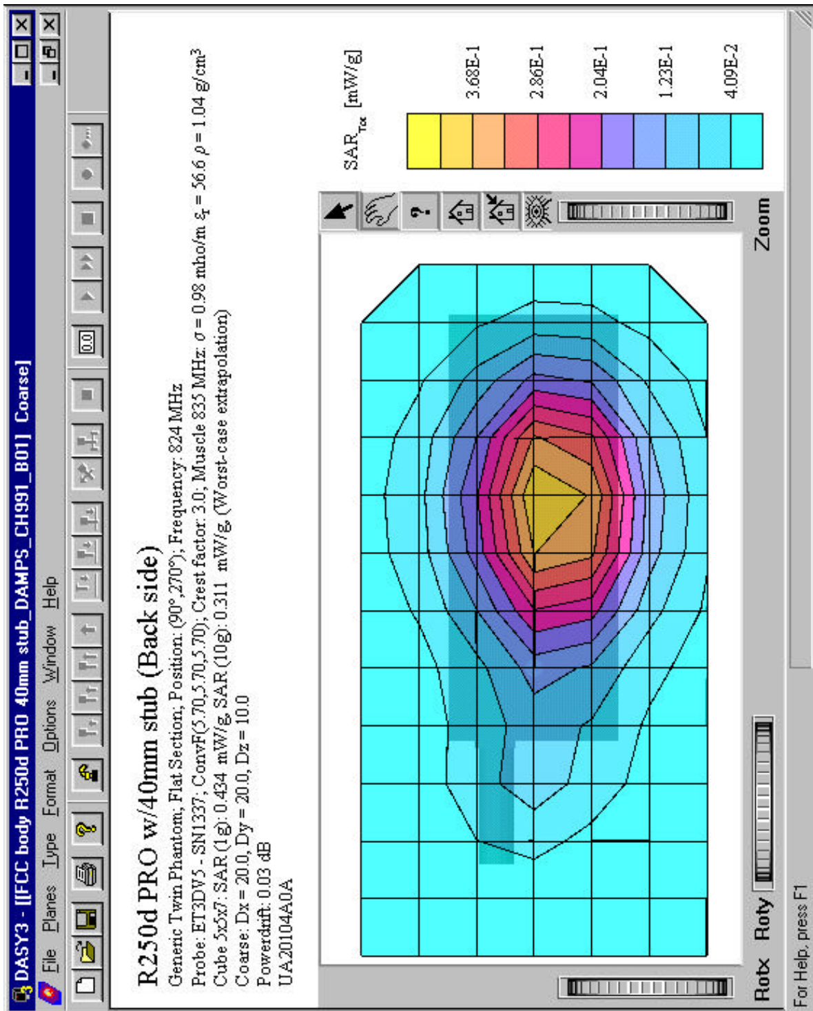
Distribution of maximum SAR in 800 TDMA band.
