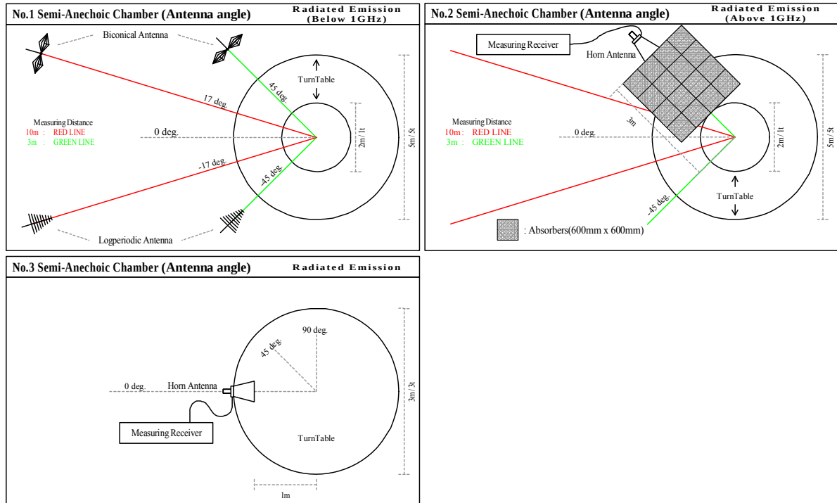
Figure 1. Antenna angle
