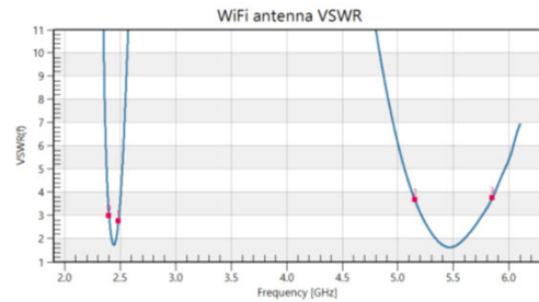
Simulated VSWR of Dual WLAN
