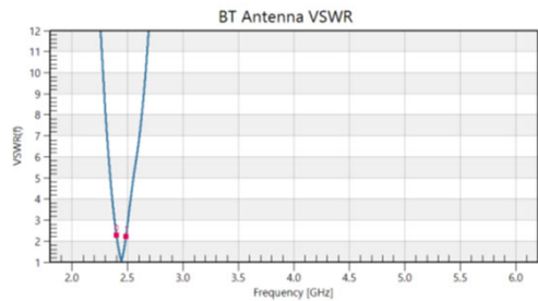
Simulated VSWR of BT
