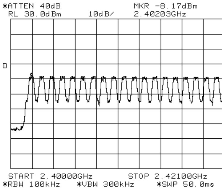
Plot 19 - Channels 0 to 18
