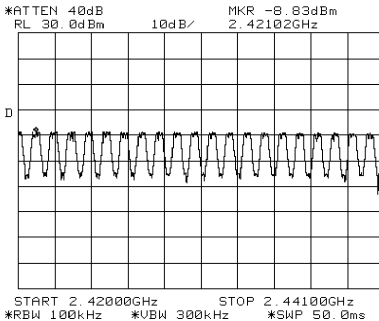
Plot 20 - Channels 19 to 38
