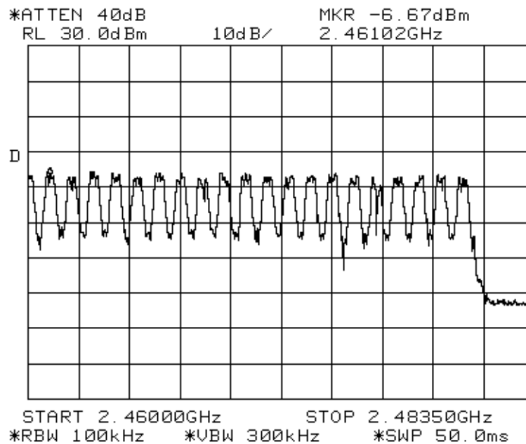
Plot 18 - Channels 59 to 78
