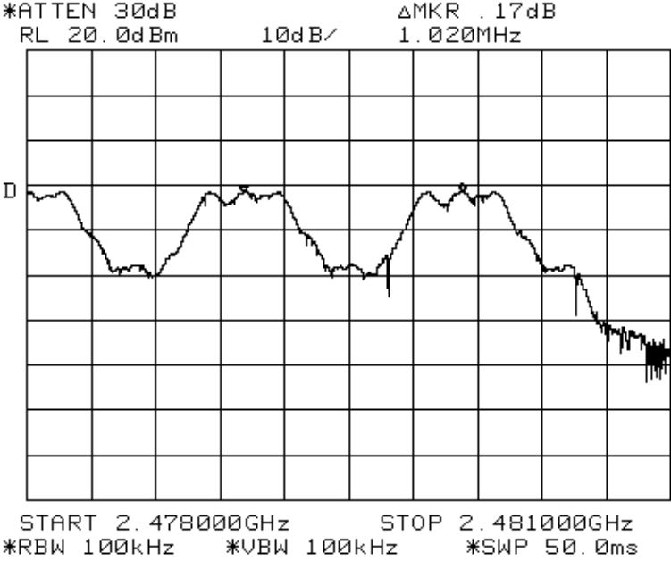
Plot 8 - Channels 77 and 78 Separation
