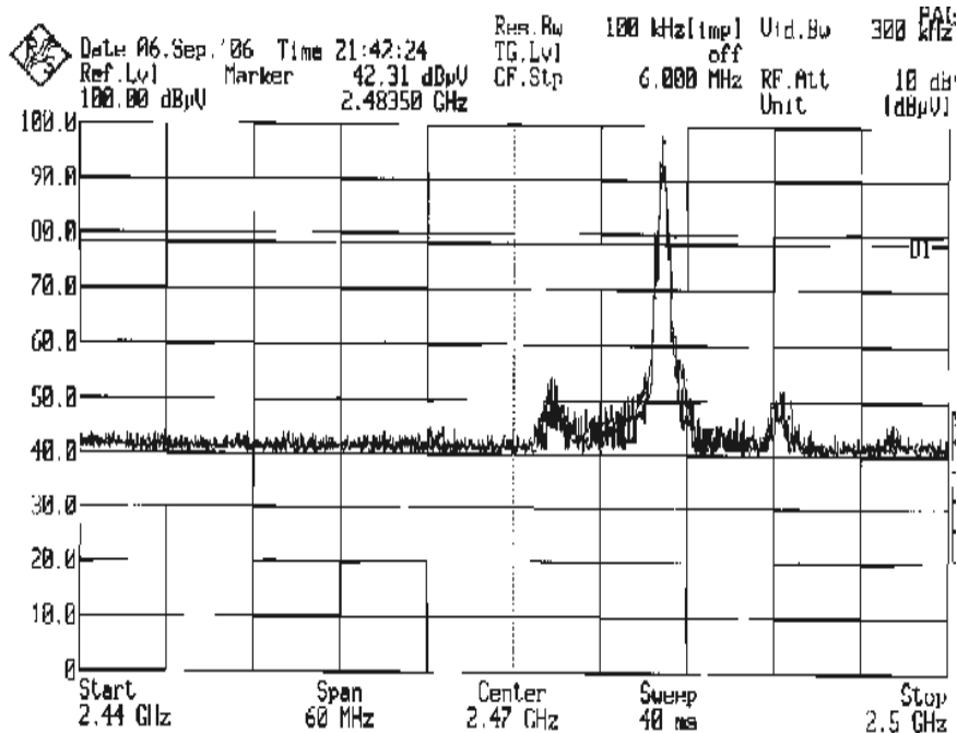
Plot 52 – Upper Band Edge at 2.4835GHz
