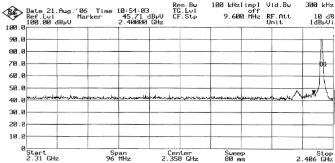
Plot 45 - Lower Band Edge at 2.4000GHz
