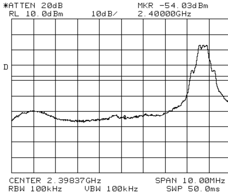
Plot 43 – Lower Band Edge at 2.4000GHz
