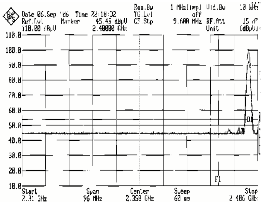
Plot 54 – Average Plot at Lower Band Edge at 2.400GHz
