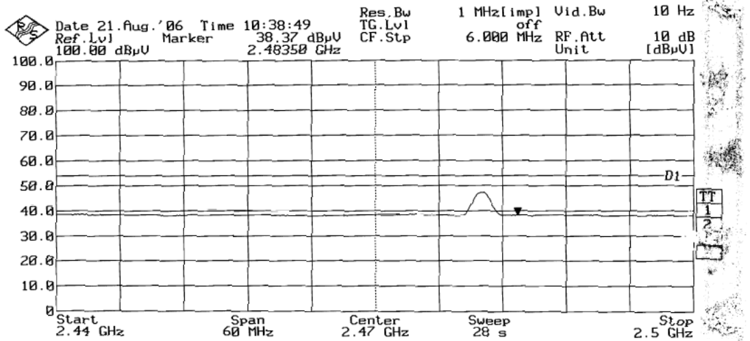
Plot 50 - Average Plot at Upper Band Edge at 2.4835GHz
