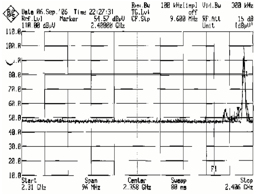
Plot 51 – Lower Band Edge at 2.4000GHz
