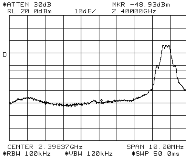
Plot 41 – Lower Band Edge at 2.4000GHz
