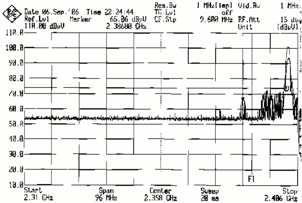
Plot 53 – Peak Plot at Lower Band Edge at 2.400GHz
