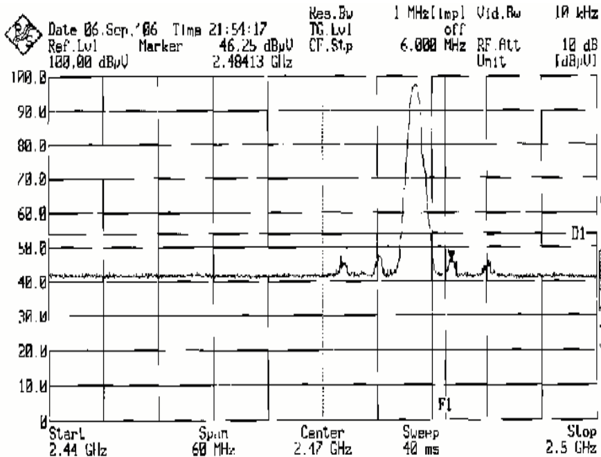
Plot 56 – Average Plot at Upper Band Edge at 2.4835GHz
