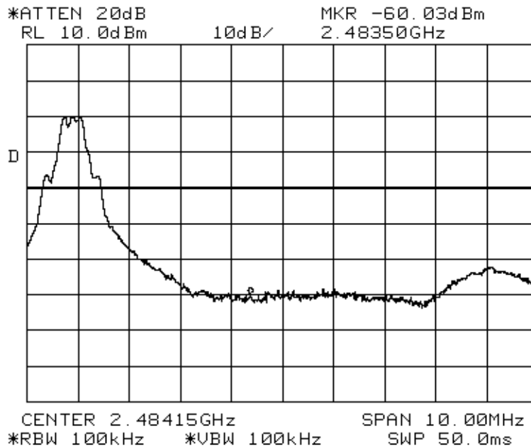
Plot 44 – Upper Band Edge at 2.4835GHz
