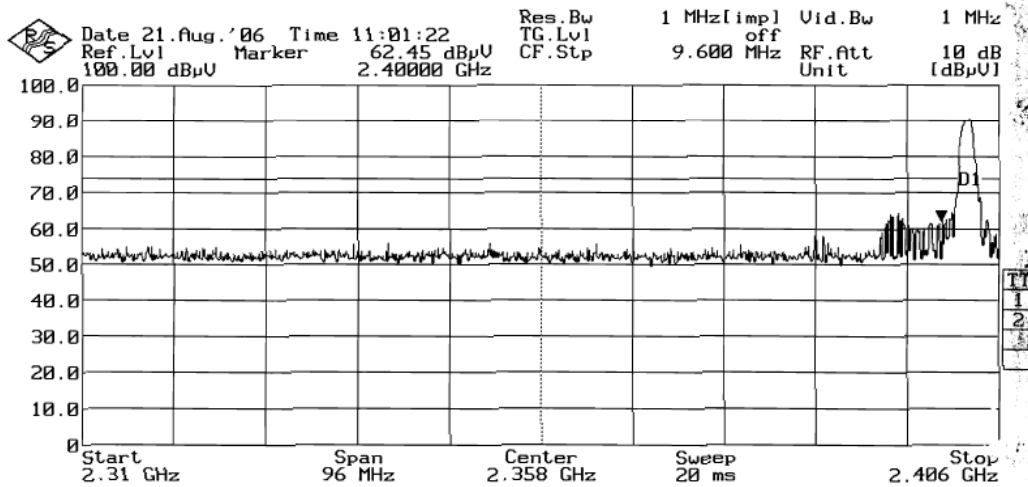
Plot 47 - Peak Plot at Lower Band Edge at 2.4000GHz
