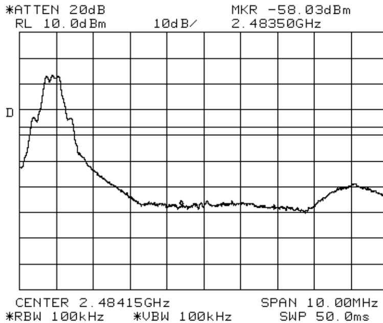
Plot 42 – Upper Band Edge at 2.4835GHz
