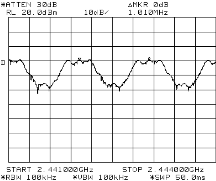
Plot 7 - Channels 39 and 40 Separation
