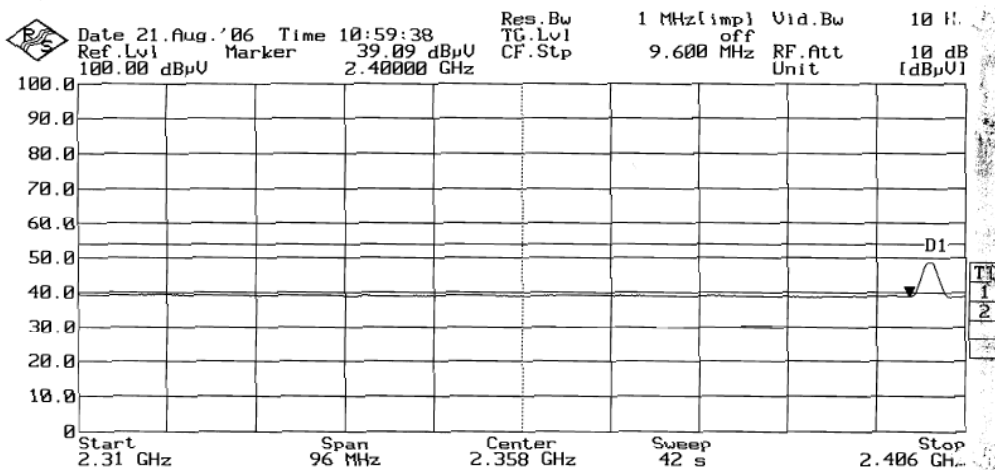
Plot 48 - Average Plot at Lower Band Edge at 2.4000GHz
