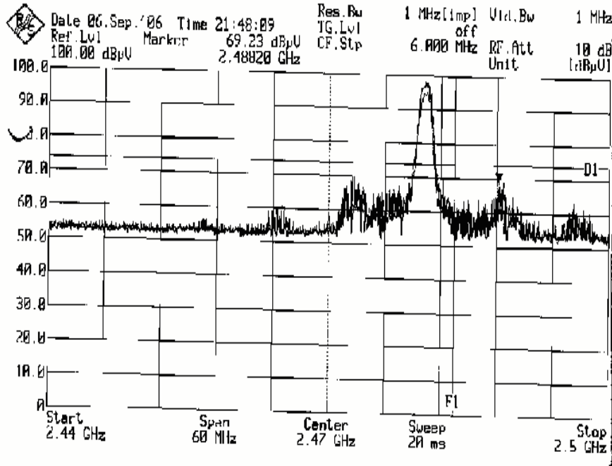
Plot 55 – Peak Plot at Upper Band Edge at 2.4835GHz
