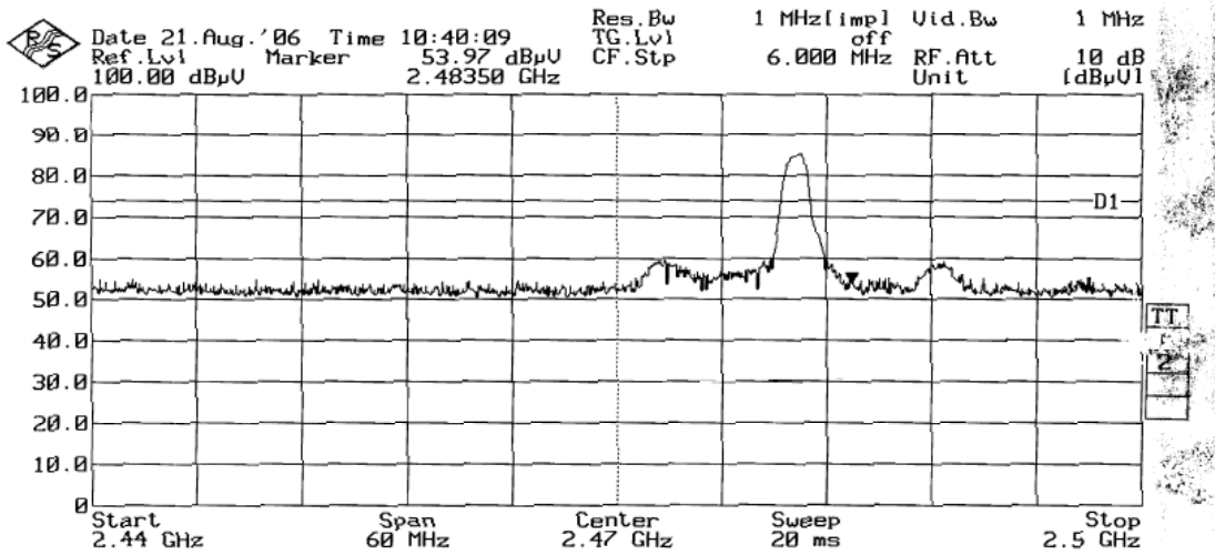
Plot 49 - Peak Plot at Upper Band Edge at 2.4835GHz
