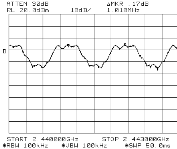
Plot 3 - Channels 39 and 40 Separation
