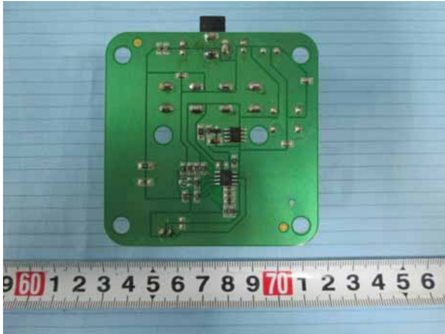
EUT – Charger Main Bottom View
