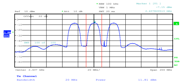
Figure 8.3-10: 802.11b power sample plot
