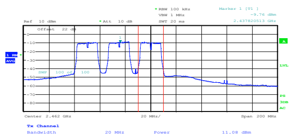
Figure 8.3-14: 802.11g power sample plot
