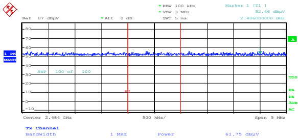
Figure 8.4-25: Intermodulation two carriers Channel 6 and 11 upper band edge Peak
