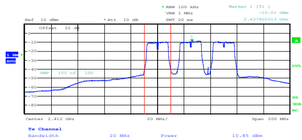
Figure 8.3-12: 802.11g power sample plot
