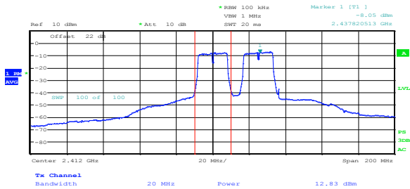
Figure 8.3-5: 802.11g power sample plot
