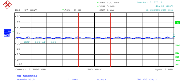
Figure 8.4-22: Intermodulation two carriers Channel 6 and 11 Low band edge Average
