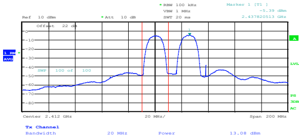
Figure 8.3-3: 802.11b power sample plot
