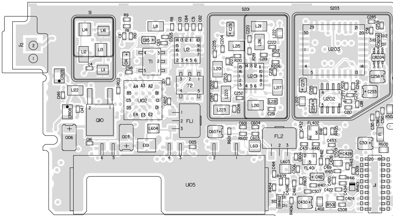
TOP VIEW
