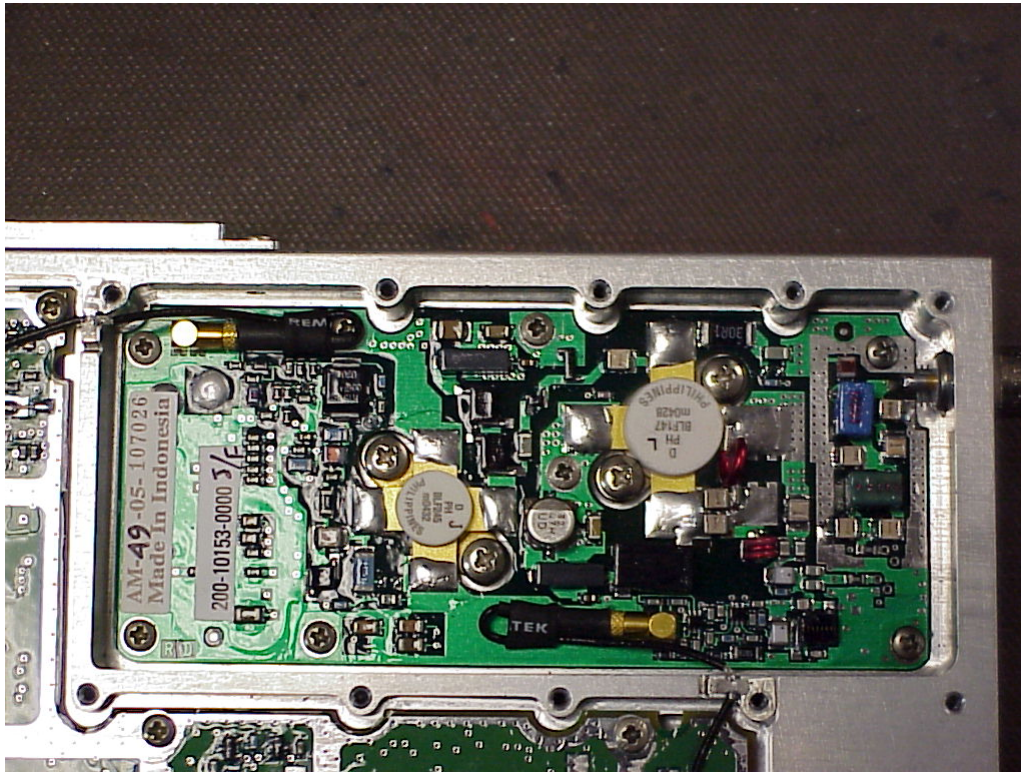
Transmitter PCB
