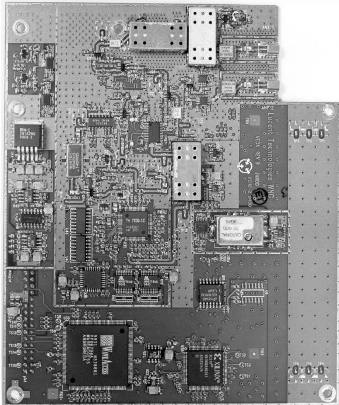
WM Radio pwb - top component side
