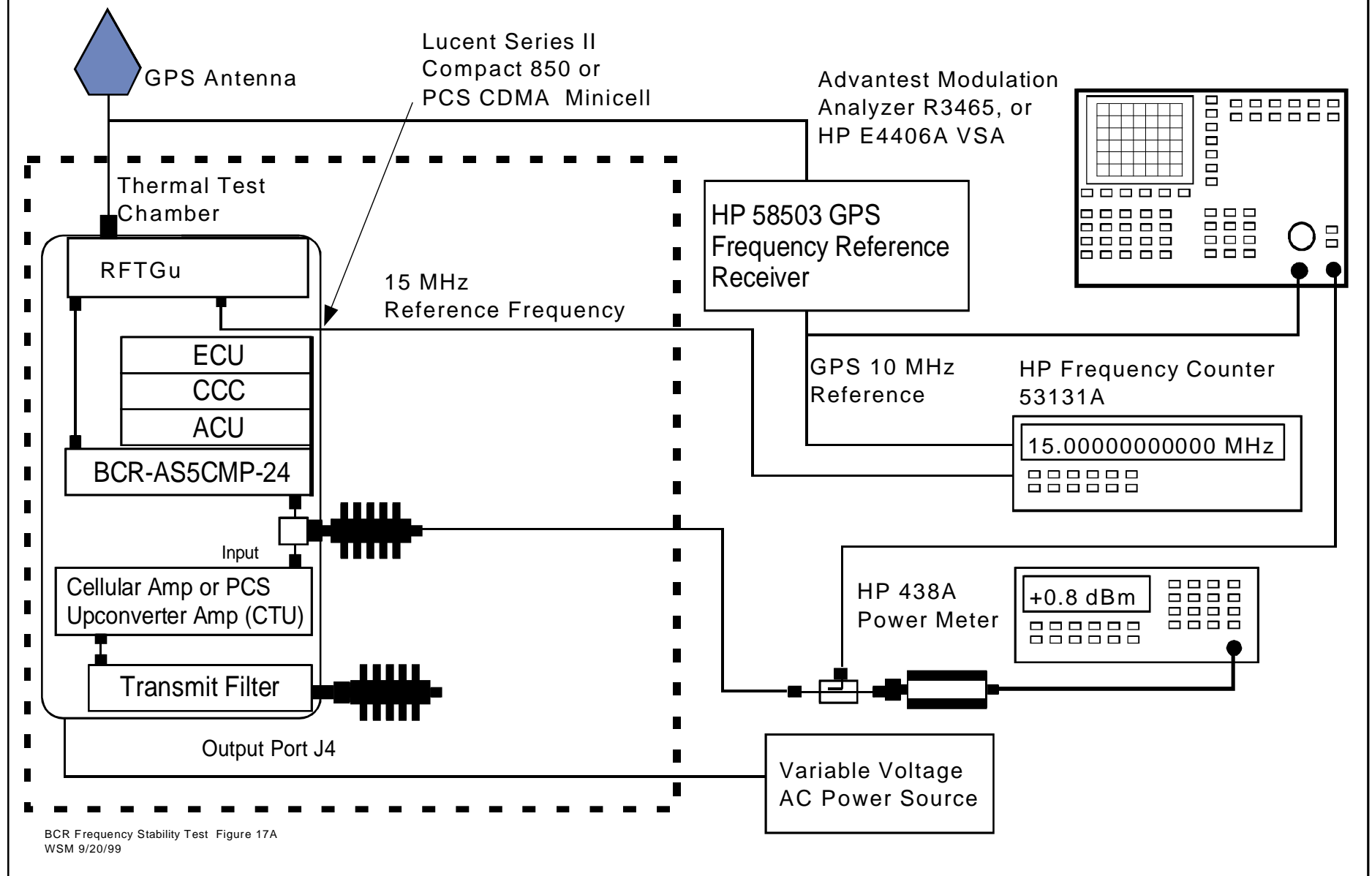
Figure 13A. Test Configuration For Frequency Stability, Modulation Quality and Power Output
