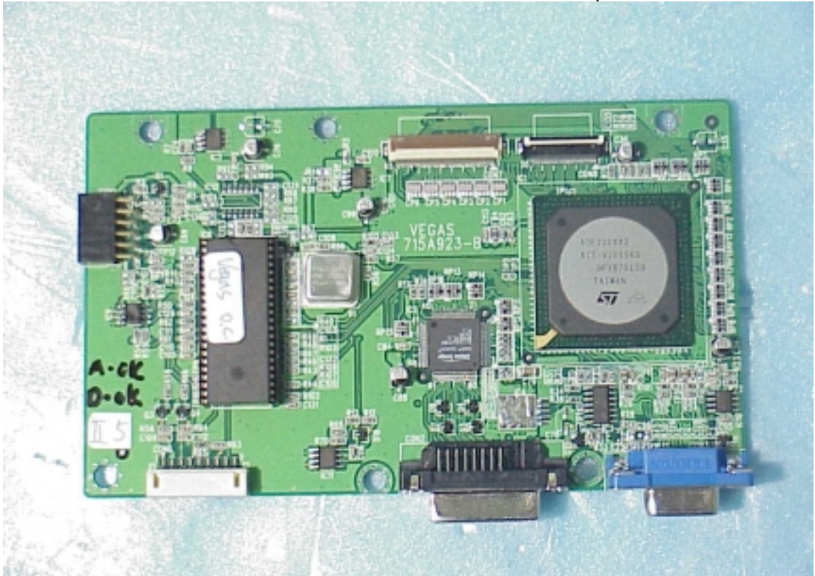
Figure 29 Frame of Internal (Main Board, Front Side)
