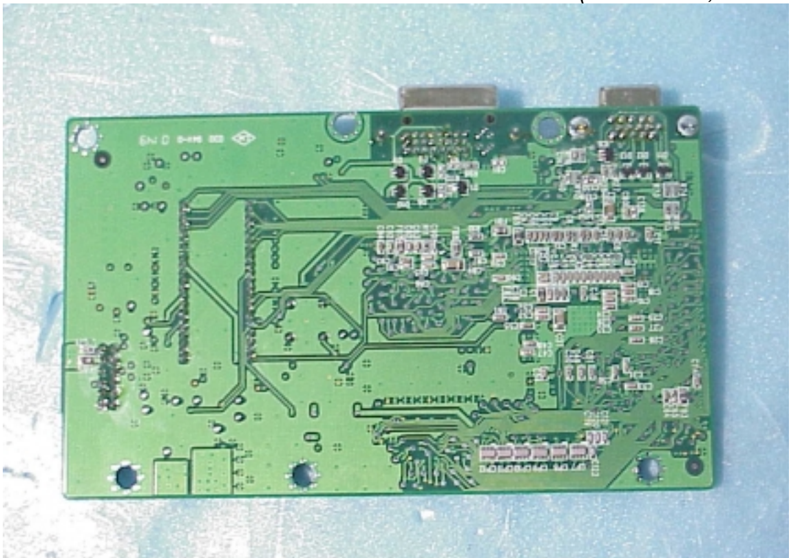
Figure 30 Frame of Internal (Main Board, Back Side)
