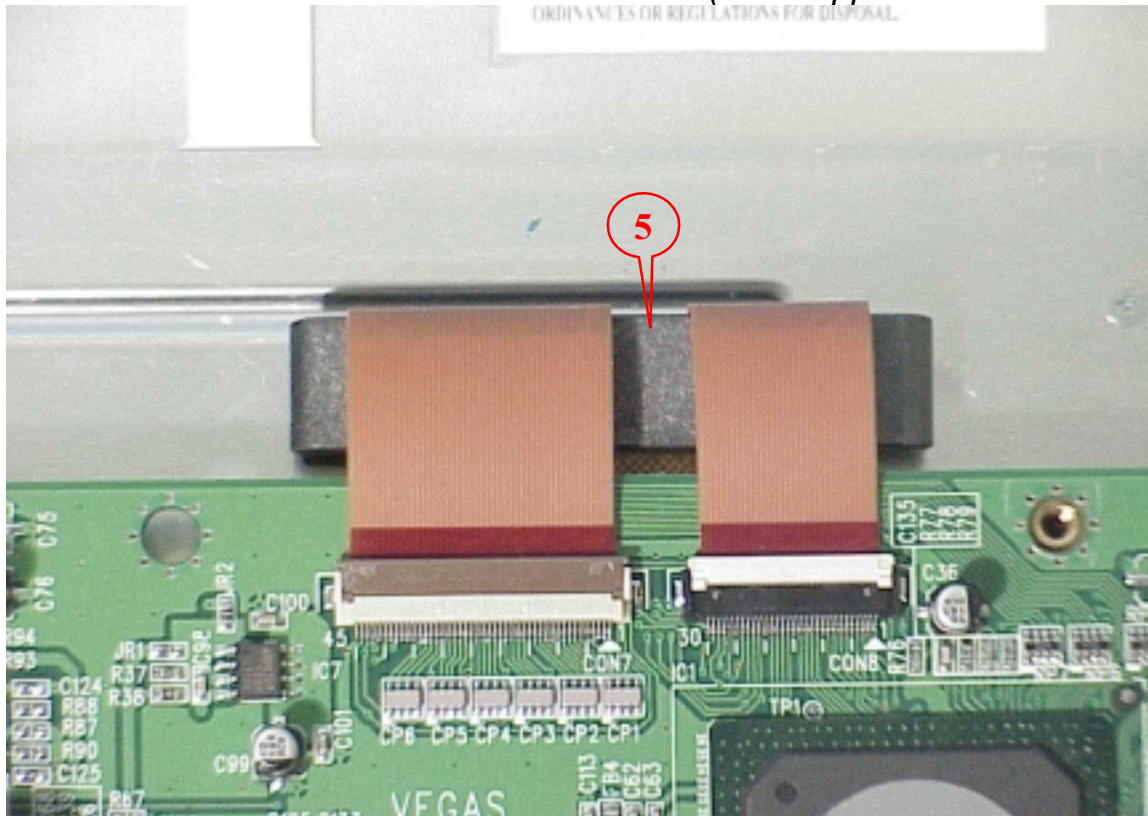
Figure 27 Frame of Internal (EMI Suppress Part-Ferrite Core)
